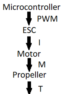
Fig. 1. : Controlled section of an UAV
