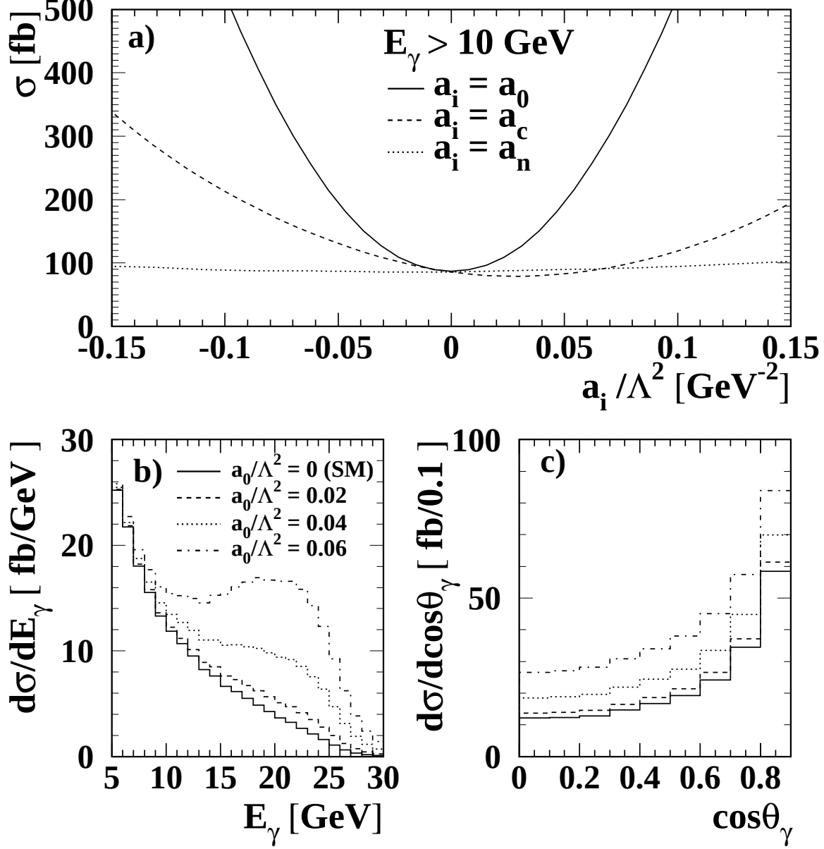
Figure 2: The effect of anomalous quartic couplings in e^+e^- collisions at \sqrt{s}=189 GeV. a) Expected W^+W^-\gamma cross-section for different anomalous quartic couplings, the photon was required to have energy, E_\gamma > 10 GeV and be within the polar acceptance, |\cos\theta_\gamma| < 0.9 . The kinematic cuts used to define the cross-section, see text, were also applied. Plots b) and c) show the effect of an anomalous quartic gauge coupling, a_0 , on the energy and angular distribution of photons in W^+W^-\gamma events, where the fiducial cuts, E_\gamma > 5 GeV and |\cos\theta_\gamma| < 0.9 were imposed. In all three figures, the contribution from final state radiation diagrams is not included.
