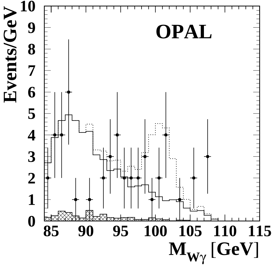
Figure 5: Reconstructed invariant mass of W^\pm\gamma in selected W^+W^-\gamma events with E_\gamma > 5 GeV (two entries per event). The 189 GeV data are shown by the points, the Standard Model expectation, determined from KORALW and PYTHIA is shown by the histogram. The shaded histogram shows the non- W^+W^-(\gamma) background. Also shown, by the dotted histogram, is the expected reconstructed mass distribution (arbitrary normalisation) for a narrow resonance of mass 100 GeV which decays to W\gamma .
