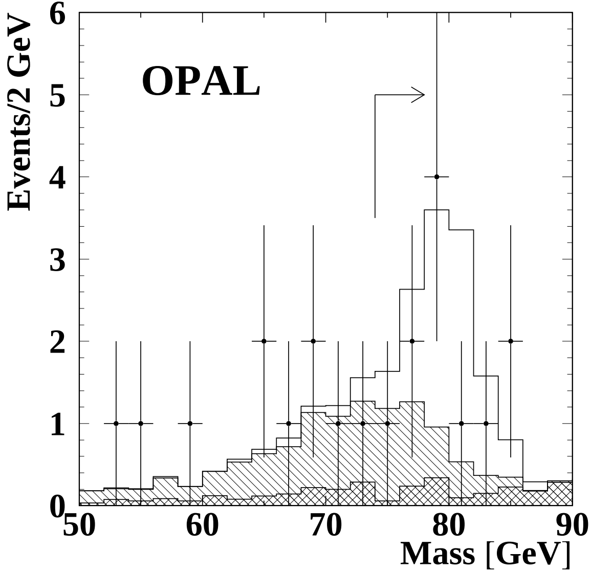
Figure 3: The reconstructed W-boson mass distribution for candidate W^+W^-(\gamma) \rightarrow q\bar{q}\ell\bar{\nu}_\ell\gamma events using the ISR/QGC hypothesis. The points show the data. The histogram shows the Monte Carlo expectation where KORALW has been used to simulate the W^+W^-(\gamma) final state and PYTHIA is used to simulate non- W^+W^- background. The hatched histogram shows the contribution from W^+W^- events with final state radiation or where the photon candidate originates from the decay of a meson. The double-hatched histogram shows the contribution from non- W^+W^- background. The cut is indicated by the arrow.
