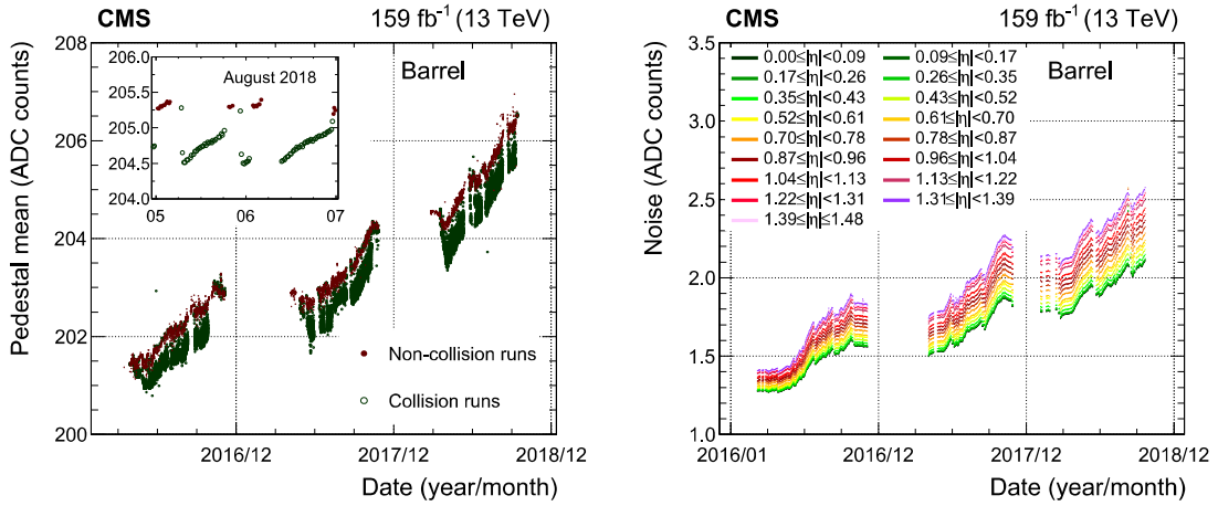
Figure 4. History of the pedestal mean value for the ECAL barrel (left) and its noise (right), measured for the highest MGPA gain in collision or noncollision runs taken during the 2016–2018 data taking period. The inset in the left panel shows an enlargement of two days in August 2018, to show in more detail the variation of the pedestal mean during LHC fills.
