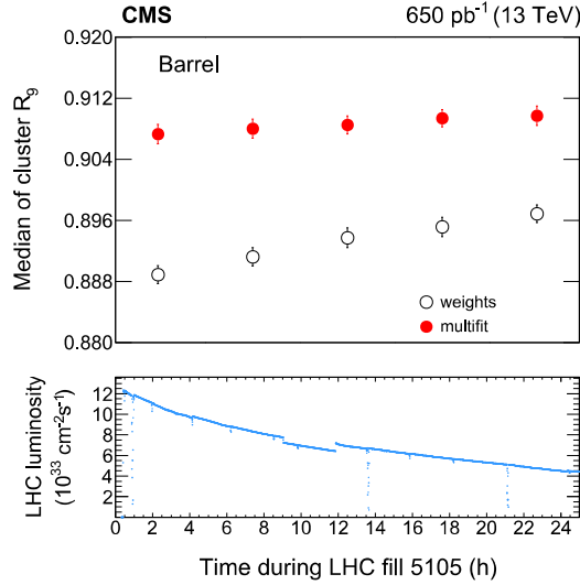
Figure 15. History of the median of the R_9 cluster shape for electrons from Z \rightarrow e^+e^- decays during one typical LHC fill in 2016. Hits are reconstructed with either the multifit (filled circles) or the weights algorithm (open circles). Each point represents the median of the distribution for a 5 hour period during the considered LHC fill. Error bars represent the statistical uncertainty on the median. The bottom panel shows the instantaneous luminosity delivered by the LHC as a function of time. The steps in the luminosity occurring about every two hours correspond to changes in the LHC beam crossing angle, which changes the overlap area of the bunches. Larger brief drops could indicate emittance scans during the fill.
