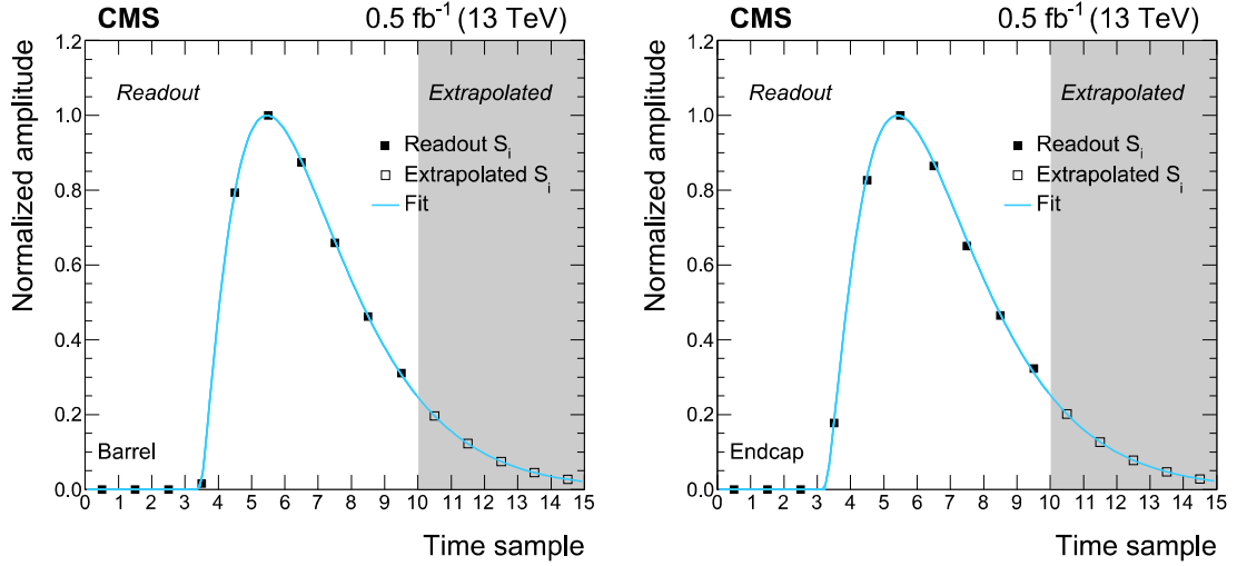
Figure 2. Pulse shape binned templates, measured in collision data recorded during June 2017 in a typical LHC fill, for a channel in the barrel (left) and in an endcap (right). The first 3 bins are the pedestal samples, and their values equal zero by construction. The following 7 bins are estimated from the average of the digitized samples on many hits, while the rightmost 5 bins are estimated by extrapolating the distribution using the function of eq. (5.1) (blue solid line).
