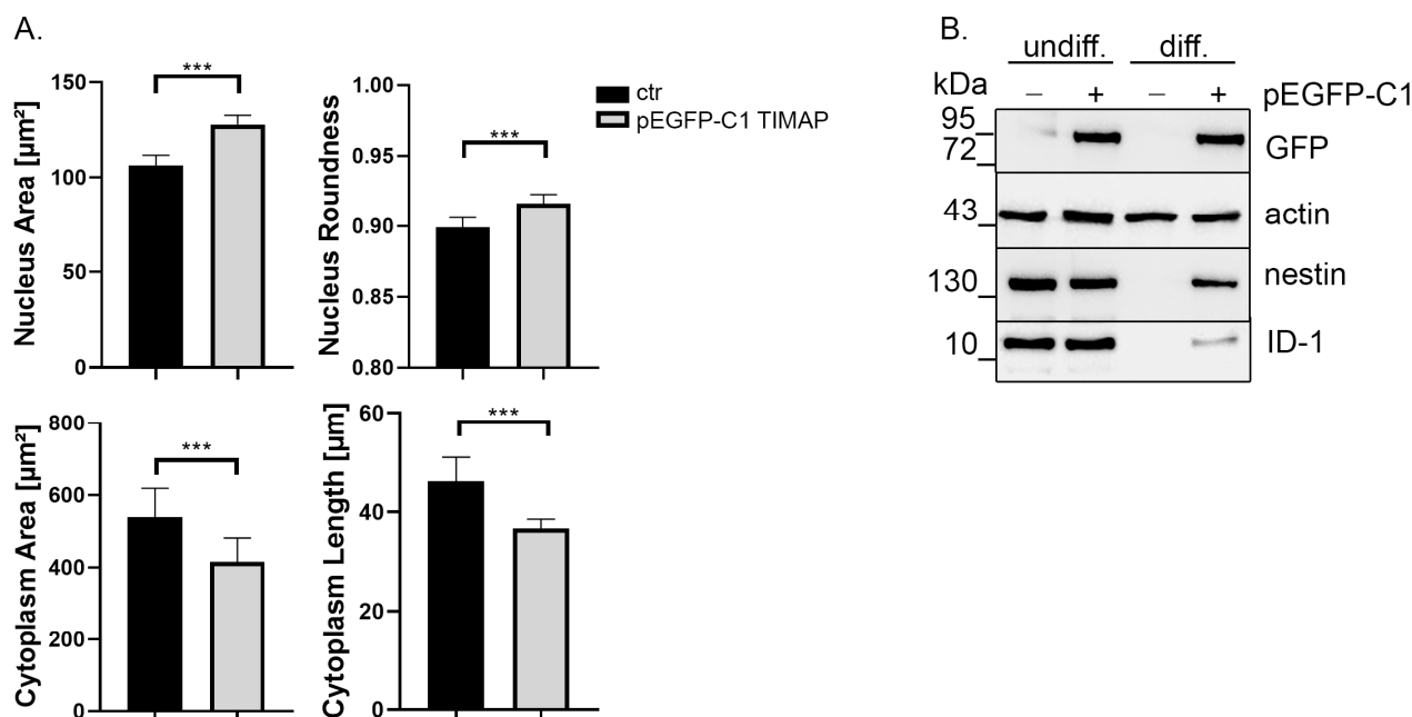
Figure 4. Overexpression of TIMAP attenuates differentiation. (A) Differentiated (Day 6) control and pEGFP-C1 TIMAP-expressing cells were analyzed using Opera Phenix HCS. Data are presented as mean \pm SD (number of cells analyzed > 1000, from n = 3 experiments). Statistical analysis was performed using unpaired t -test (** p < 0.001 ). (B) Control or pEGFP-C1 TIMAP-expressing cells were treated with vehicle (DMSO) (undiff) or ATRA (diff) for 6 days. Samples were tested using GFP-, nestin-, ID-1- and actin (loading control)-specific antibodies.
