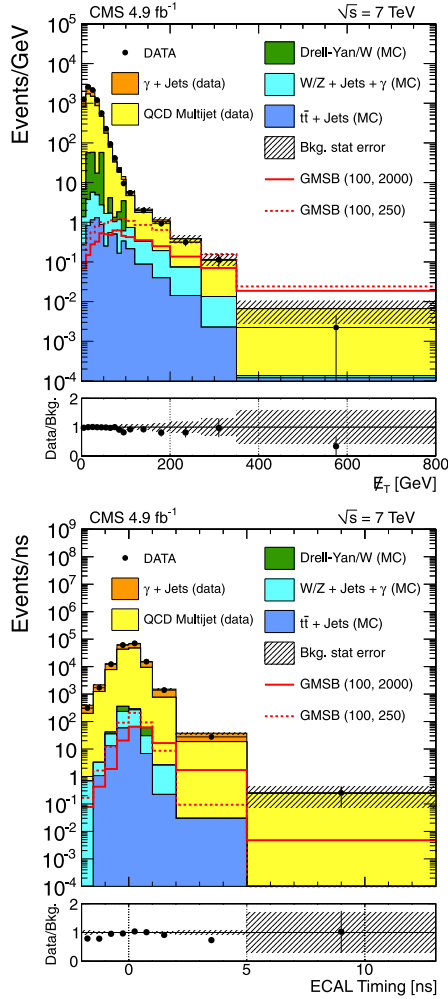
Fig. 5. The one-dimensional projection for E_T (top) and for ECAL timing (bottom), after all selection requirements. The multijet and \gamma + jets backgrounds are normalized to the yields from the fit. The rest of the backgrounds are fixed according to the integrated luminosity of the data. The GMSB (100, 2000) benchmark point corresponds to \Lambda = 100 TeV, c\tau = 2000 mm and the GMSB (100, 250) benchmark point corresponds to \Lambda = 100 TeV, c\tau = 250 mm. (For interpretation of the references to color in this figure legend, the reader is referred to the web version of this Letter.)
