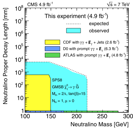
Fig. 8. The observed exclusion region for the mass and proper decay length of the long-lived \tilde{\chi}_1^0 in the SPS8 model of GMSB supersymmetry. (For interpretation of the references to color in this figure legend, the reader is referred to the web version of this Letter.)
