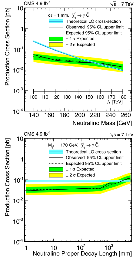
Fig. 7. Upper limits at the 95% CL on the cross section as a function of the \tilde{\chi}_1^0 mass for \tau = 1 mm (top), and for the \tilde{\chi}_1^0 proper decay length for M_{\tilde{\chi}_1^0} = 170 GeV (bottom) in the SPS8 model of GMSB supersymmetry. (For interpretation of the references to color in this figure legend, the reader is referred to the web version of this Letter.)
