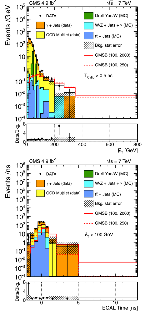
Fig. 6. The one-dimensional projection after all selection requirements for E_T for events with T_{\text{calib}} > 0.5 ns (top) and for ECAL timing (bottom) for events with E_T > 100 GeV. The multijet and \gamma + jets backgrounds are normalized to the yields from the fit. The rest of the backgrounds are fixed according to the integrated luminosity of the data. The GMSB (100, 2000) benchmark point corresponds to \Lambda = 100 TeV, c\tau = 2000 mm and the GMSB (100, 250) benchmark point corresponds to \Lambda = 100 TeV, c\tau = 250 mm. (For interpretation of the references to color in this figure legend, the reader is referred to the web version of this Letter.)
