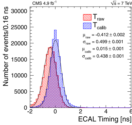
Fig. 2. The ECAL timing distribution for data, before and after calibration, overlaid with the results of the Gaussian fits.
