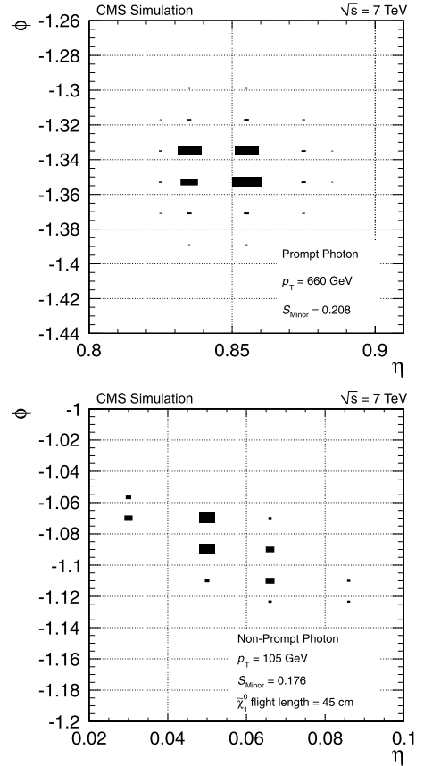
Fig. 3. The distribution of energy deposition in the ECAL crystals for a prompt (top) and a non-prompt (bottom) photon. Each rectangle represents an ECAL crystal and has a size that is proportional to the energy deposited in that crystal. The non-prompt illustration is for a \chi^0_1 flight length of 45 cm.
