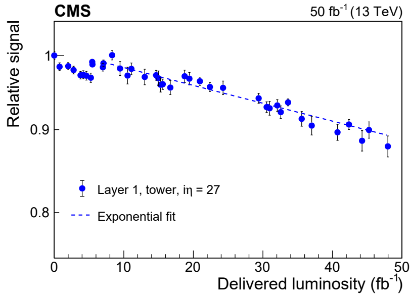
Figure 9. Relative signal measured using the laser calibration system versus delivered luminosity for the SCSN–81 tile in layer 1 with i\eta = 27 and i\phi = 63 . Scaled statistical uncertainties are shown (see text). For this tile, the estimated dose at the end of data taking was d = 1.5 kGy, and the average dose rate was R = 0.89 Gy/h. The dashed line represents a fit to the data to obtain the value of the exponential slope. Note that the vertical scale is logarithmic (base 10).
