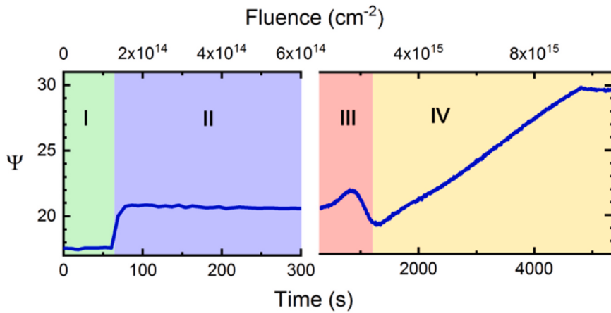
Fig. 4. Evolution of the ellipsometric angle \Psi measured in-situ at the wavelength of 450 nm during the implantation of 200-keV \text{Sb}^+ ions into c-Ge. The four dominant regions of structural changes are numbered and marked by different background colors. The regions represent (I) the baseline for the unimplanted case (II) the damage accumulation and amorphization (III) the rapid void formation and (IV) the period of slow change of damage and void constituents. Note the different time for scale of regions (I) and (III) for a better visualization of the transient at \approx 60 s, i.e., the starting point of the implantation.
