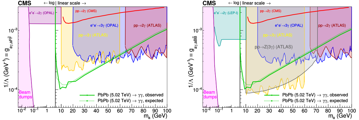
Fig. 7. Exclusion limits at 95% CL in the ALP-photon coupling g_{a\gamma} versus ALP mass m_a plane, for the operators a\tilde{F}F/4\Lambda (left, assuming ALP coupling to photons only) and aB\tilde{B}/(4\Lambda\cos^2\theta_W) (right, including also the hypercharge coupling, thus processes involving the Z boson) derived in Refs. [30,56] from measurements at beam dumps [60], in e^+e^- collisions at LEP-I [56] and LEP-II [57], and in pp collisions at the LHC [13,58,59], and compared to the present PbPb limits.
