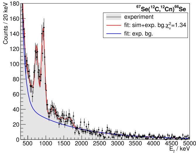
Fig. 1. Doppler-corrected singles \gamma -ray spectrum for ^{66}\text{Se} using addback procedure for the ^{67}\text{Se}(^{12}\text{C}, ^{12}\text{Cn})^{66}\text{Se} reaction channel. The data with error bars and shaded area represent the experimental spectrum, the red line is the simulation plus a double-exponential background, and the latter function (exponential background) is also plotted separately as a blue line.
