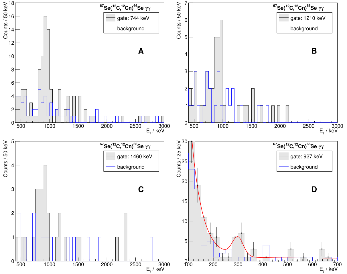
Fig. 2. Doppler-corrected coincidence \gamma -ray spectra for ^{66}\text{Se} using addback procedure for the ^{67}\text{Se}(^{12}\text{C},^{12}\text{Cn})^{66}\text{Se} reaction channel. The data with a grey shaded area represent the experimental spectrum by selecting events in the \gamma\gamma matrices in coincidence with a prompt \gamma ray, while the blue background spectrum was created by selecting a gate right beside the prompt \gamma ray in question. A: events coincident with the 744-keV transition, B: events coincident with the 1210-keV transition, C: events coincident with the 1460-keV transition, D: low-energy events coincident with the 927-keV transition; the red line is the simulation plus a double-exponential background.
