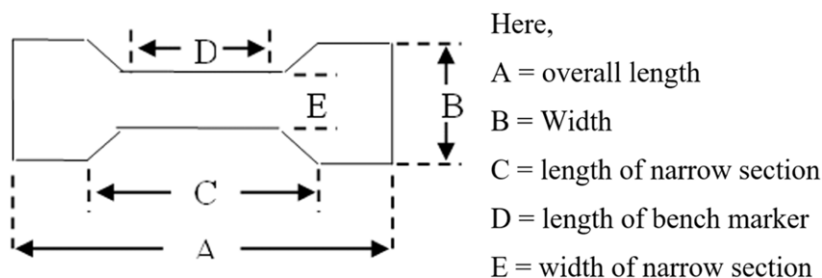
Figure 2. Dumbbell-shape specimen for tensile test.
