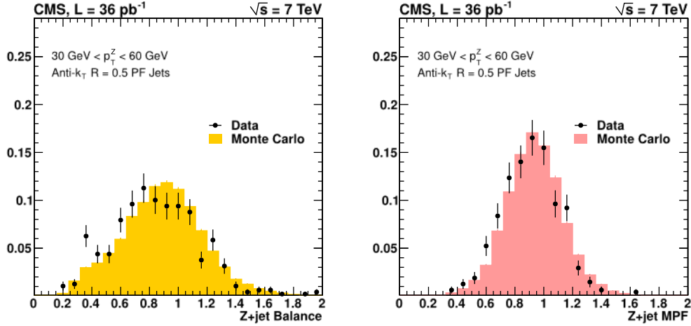
Figure 18. Left: jet energy response from Z(\mu^+\mu^-)+\text{jets} p_T -balancing in the bin 30 < p_T^Z < 60 GeV. Right: jet energy response from Z(\mu^+\mu^-)+\text{jets} MPF in the bin 30 < p_T^Z < 60 GeV.
