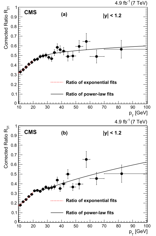
Fig. 3. Measured differential cross section ratios as a function of p_T . Corrected yield ratios: (a) R_{21} ; (b) R_{31} . The dashed line is the ratio of the exponential fits to the individual differential cross sections for 10 < p_T < 20 GeV. The solid line is the ratio of the corresponding power-law fits for p_T > 20 GeV.
