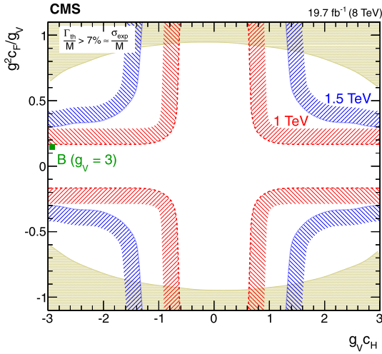
Fig. 7. Exclusion regions in the plane of the HVT-model coupling constants ( g_{VC_H} , g^2 C_F/g_V ) for two resonance masses, 1.0 and 1.5 TeV. The point B of the benchmark model used in the analysis, corresponding to g_V = 3 and C_F = -C_H = 1 , is also shown. The boundaries of the regions of the plane excluded by this search are indicated by the dashed and dotted lines, and associated hatching. The areas indicated by the solid line and solid shading correspond to regions where the theoretical width is larger than the experimental resolution of the present search and thus the narrow-resonance assumption is not satisfied.
