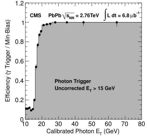
Fig. 1. Efficiency for the photon trigger as a function of the corrected photon transverse energy in PbPb collisions at 2.76 TeV, measured with the minimum-bias sample. Error bars represent the statistical uncertainty.
