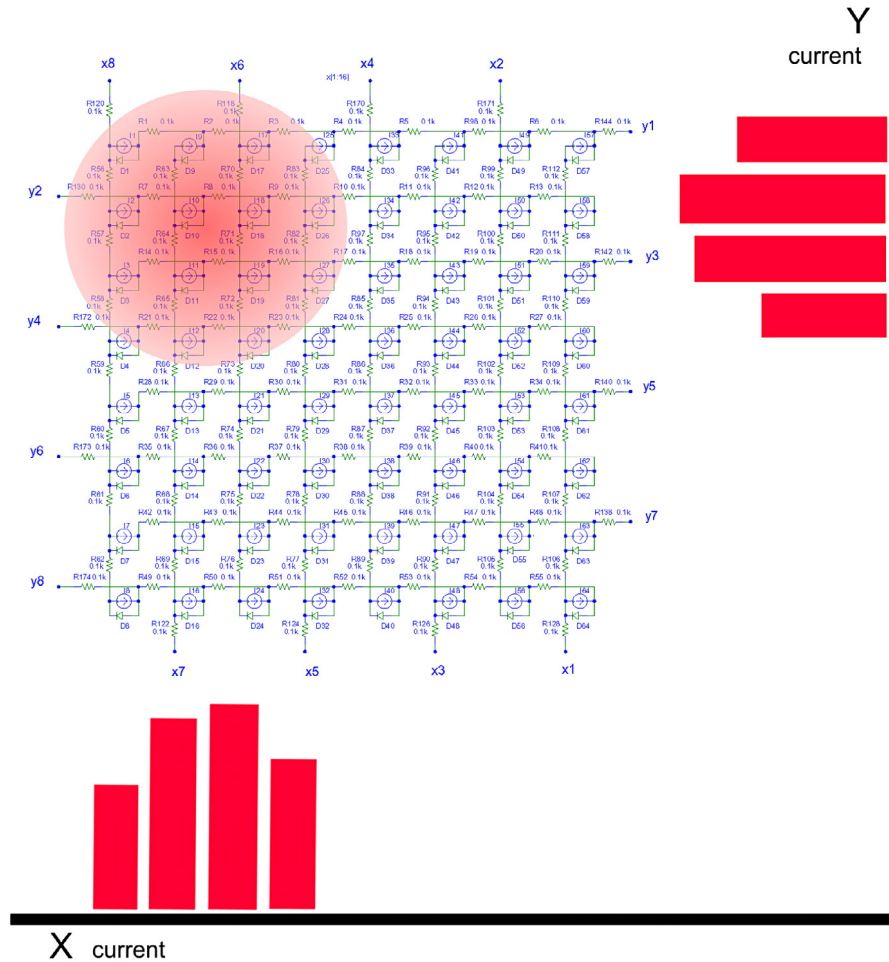
Fig. 5. Example of the electronic equivalence of an 8 \times 8 strips ASPD sensor, with a sketch of the readout current distributions generated by a light spot illuminating 4 strips in each direction.
