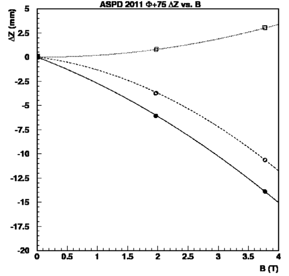
Fig. 25. During ramp up in magnet intensity in 2011: motion \Delta Z (LD-AR) (dots), \Delta Z (LD&TP) with respect to the Interaction Point as seen from P2 in the laser path L2 (circles) and motion of ME/1/2 with respect to LD as seen from P5 in the laser path L4 (squares).
