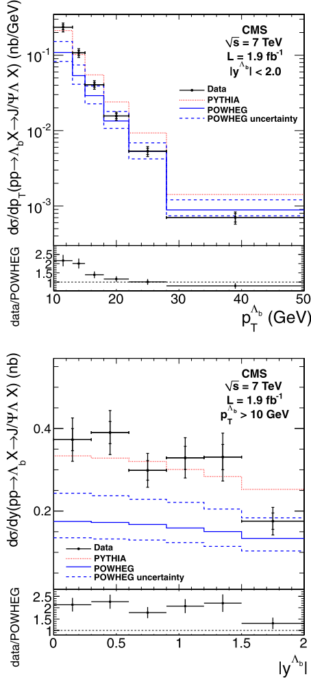
Fig. 2. Upper: Measured differential cross sections times branching fraction d\sigma/dp_T^{\Lambda_b} \times B(\Lambda_b \rightarrow J/\psi \Lambda) (top) and d\sigma/dy^{\Lambda_b} \times B(\Lambda_b \rightarrow J/\psi \Lambda) (bottom) compared to the theoretical predictions from PYTHIA and POWHEG . The inner error bars correspond to the statistical uncertainties and the outer ones represent the uncorrelated systematic uncertainties added in quadrature to the statistical uncertainties. The dashed lines show the uncertainties on the POWHEG predictions. Overall uncertainties of 2.2% for the luminosity and 1.3% for the J/\psi \rightarrow \mu^+ \mu^- and \Lambda \rightarrow p\pi branching fractions for the data are not shown, nor is the 54% uncertainty due to B(\Lambda_b \rightarrow J/\psi \Lambda) for the PYTHIA and POWHEG predictions. Lower: The ratio of the measured values to the POWHEG predictions. The error bars include the statistical and uncorrelated systematic uncertainties on the data and the shape-only uncertainties on the POWHEG predictions.
