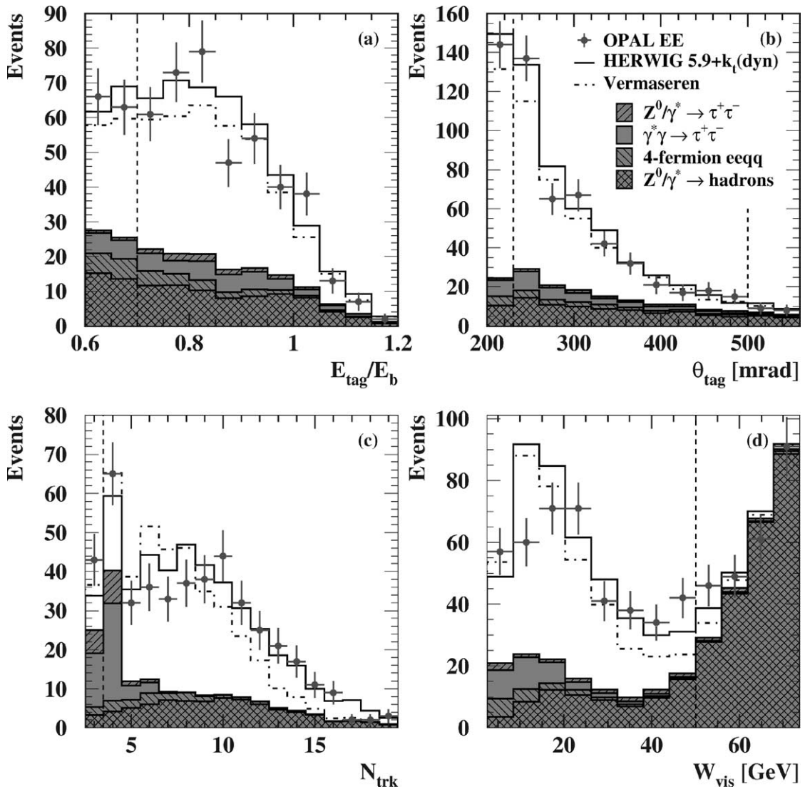
Fig. 2. Comparison of data distributions for the EE sample with the Monte Carlo predictions. See Fig. 1 for details.
