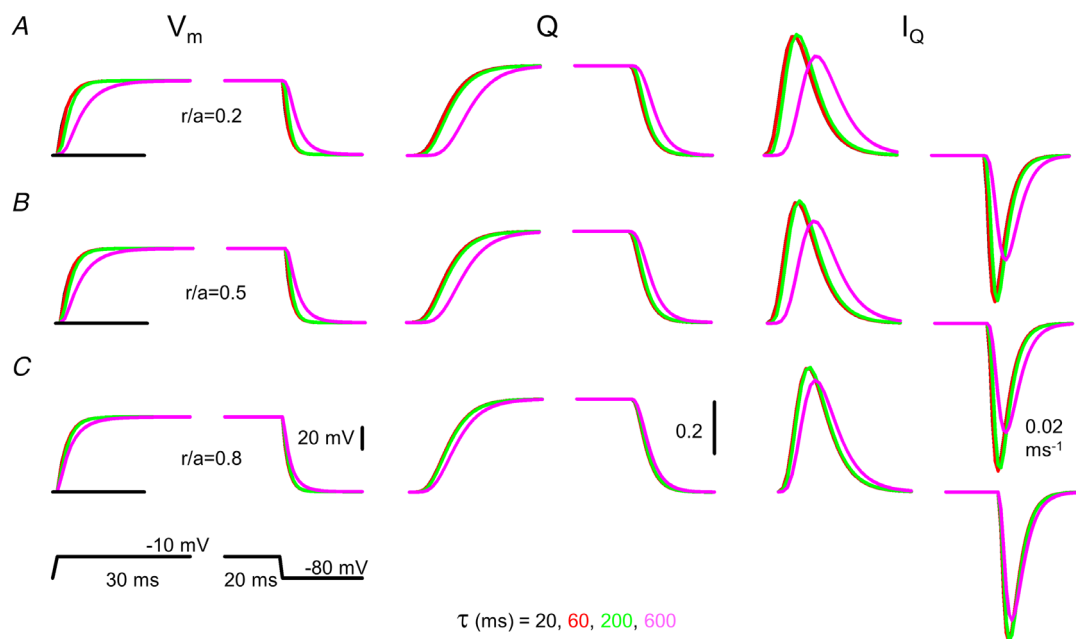
Figure 3. Simulated time courses of membrane potential ( V_m ), charge in the activating position ( Q ) and charge movement current ( I_Q )
