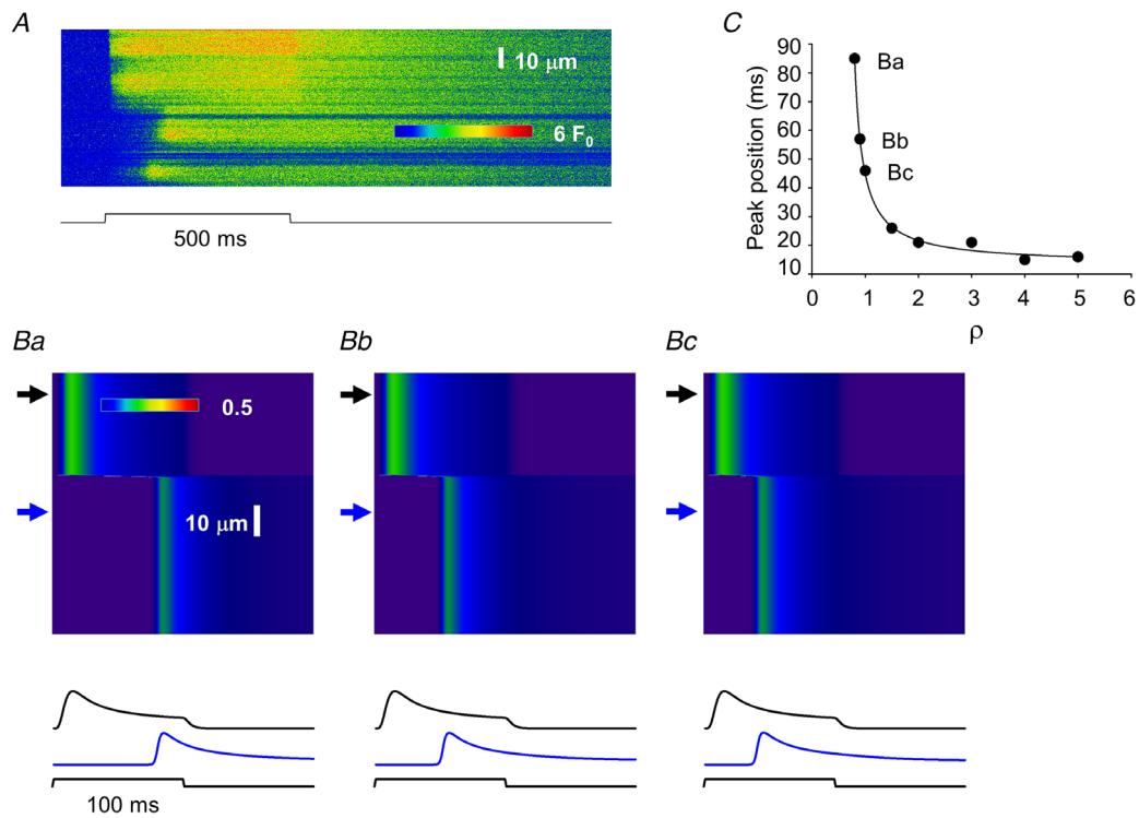
Figure 10. Simulation of delayed activation in MTM1-deficient muscle fibres
