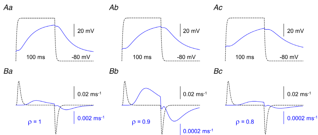
Figure 11. Simulated changes in membrane potential and intramembrane charge movement
