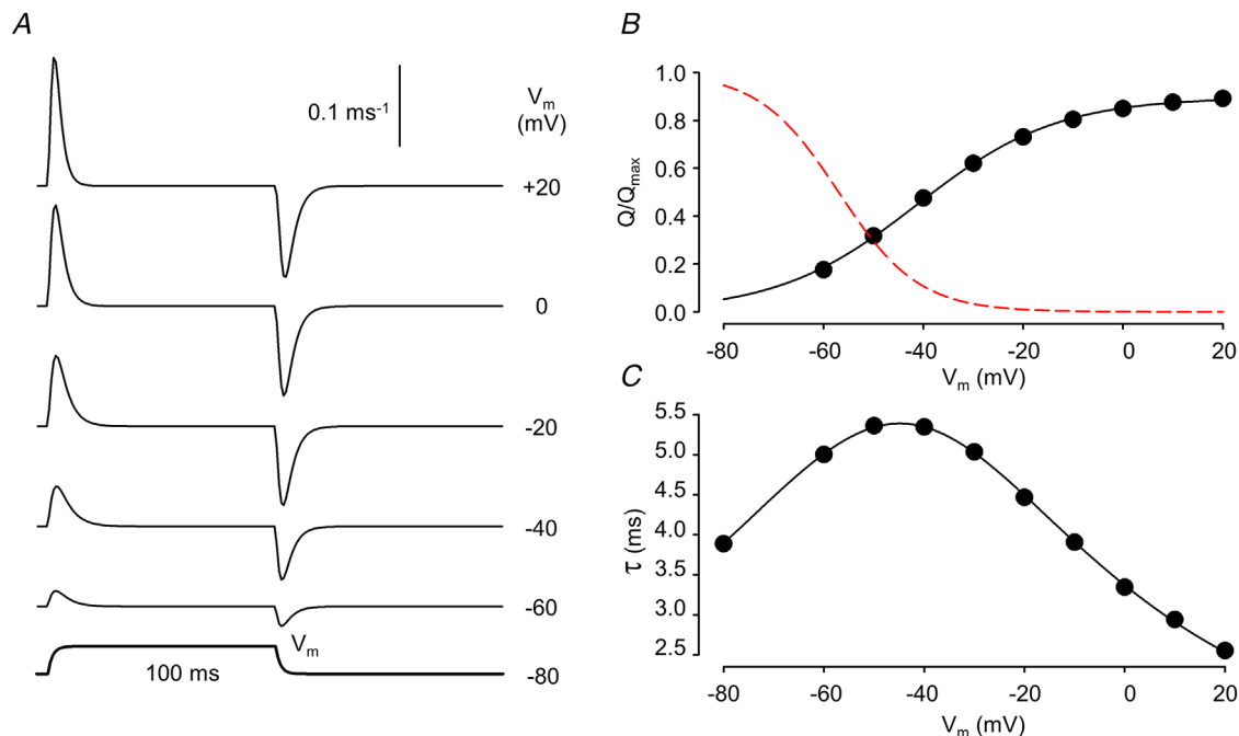
Figure 1. Voltage dependence of intramembrane charge movement
