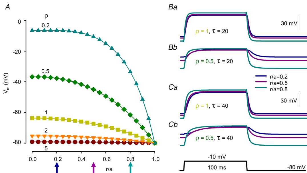
Figure 2. Simulated profiles of membrane potentials with different T-tubule parameters
