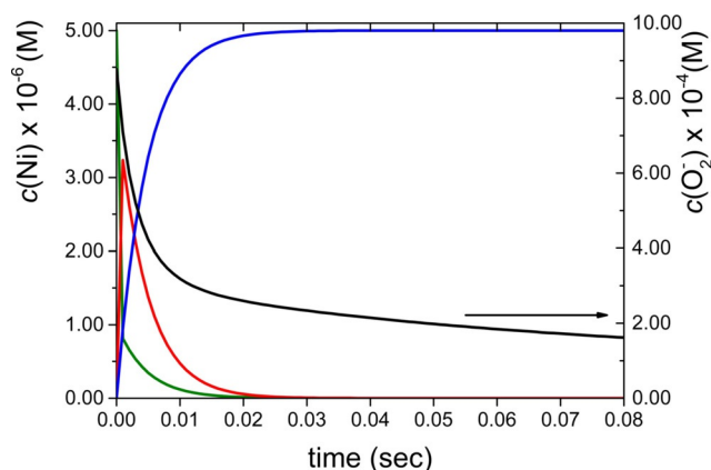
Figure 6. Calculated concentration profiles of each species as a function of time. Green: \text{Ni}^{\text{II}}_2\text{L} ; red: \text{Ni}^{\text{III}}_2\text{L} ; blue: \text{Ni}^* ; black: \text{O}_2^- . c(\text{Ni}^{\text{II}}_2\text{L})^0 = 5 \mu\text{M} , c(\text{O}_2^-)^0 = 877 \mu\text{M} .
