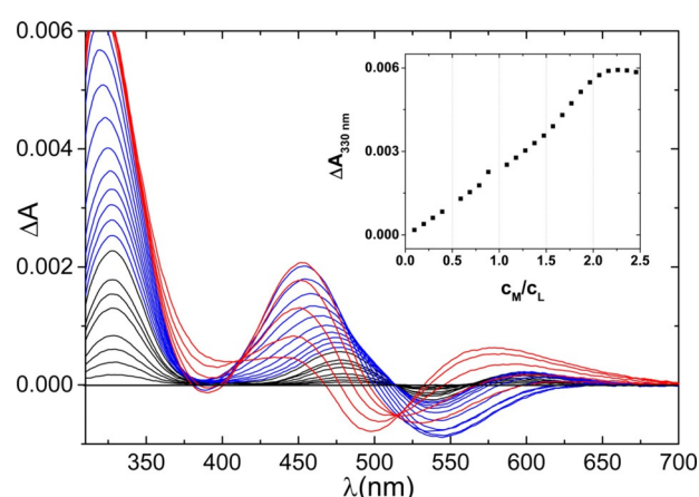
Figure 1. CD titration of L with \text{Ni}^{\text{II}} at pH 7.6. The spectra in black correspond to the samples between 0 and 1 equivalent of \text{Ni}^{\text{II}} per L , the spectra in blue correspond to the samples between 1 and 2 equivalent of \text{Ni}^{\text{II}} per L and the spectra in red correspond to the samples between 2 and 2.5 equivalent of \text{Ni}^{\text{II}} per L . Inset: evolution of \Delta A at 330 nm. c_L=1.1 mM.
