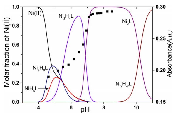
Figure 2. Distribution of the complexes formed in the \text{Ni}^{\text{II}}/\text{L} 2:1 system and the absorbance at 450 nm obtained by UV/Vis spectroscopy as a function of pH ( I = 0.2\text{ M KCl} , T = 298\text{ K} ). c_{\text{Ni(II)}} = 2.4\text{ mM} .
