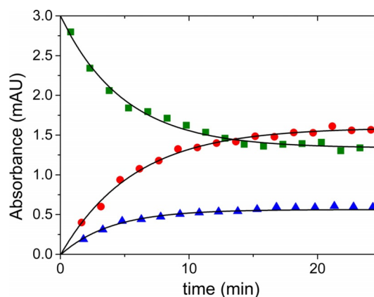
Figure 3. The decay of the concentration of the free ligand (■) and simultaneous formation of complexes \text{NiL} (●) and \text{Ni}_2\text{L} (▲) as a function of time at 0.9:1 metal to ligand ratio (pH 9.0). These time profiles were recorded in designated CE experiments (cf. experimental details) and were fitted by a single exponential function (solid line). c_{\text{L}} = 42\text{ }\mu\text{M} .
