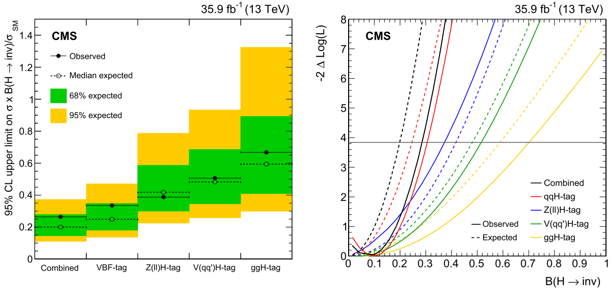
Fig. 8. On the left, observed and expected 95% CL upper limits on (\sigma/\sigma_{\text{SM}}) \mathcal{B}(H \rightarrow \text{inv}) for both individual categories targeting VBF, Z(\ell\ell) H, V(qq') H, and ggH production mode, as well as their combination, assuming an SM Higgs boson with a mass of 125.09 GeV. On the right, profile likelihood ratios as a function of \mathcal{B}(H \rightarrow \text{inv}) . The solid curves represent the observations in data, while the dashed lines represent the expected result from a b-only fit. The observed and expected likelihood scans are reported for the full combination, as well as for the individual VBF, Z(\ell\ell) H, V(qq') H and ggH-tagged analyses.
