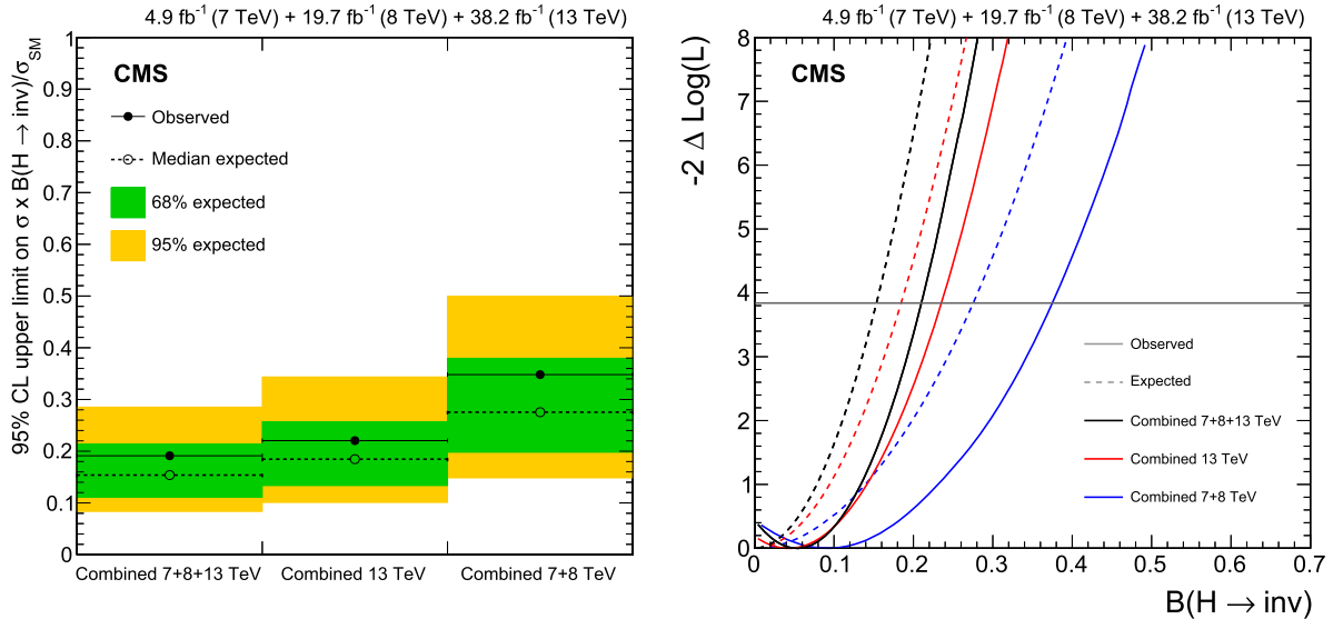
Fig. 9. On the left, observed and expected 95% CL upper limits on (\sigma/\sigma_{\text{SM}}) \mathcal{B}(H \rightarrow \text{inv}) for partial combinations based either on 7+8 or 13 TeV data as well as their combination, assuming SM production cross sections for the Higgs boson with mass of 125.09 GeV. On the right, the corresponding profile likelihood ratios as a function of \mathcal{B}(H \rightarrow \text{inv}) are presented. The solid curves represent the observations in data, while the dashed lines represent the expected result obtained from the background-only hypothesis.
