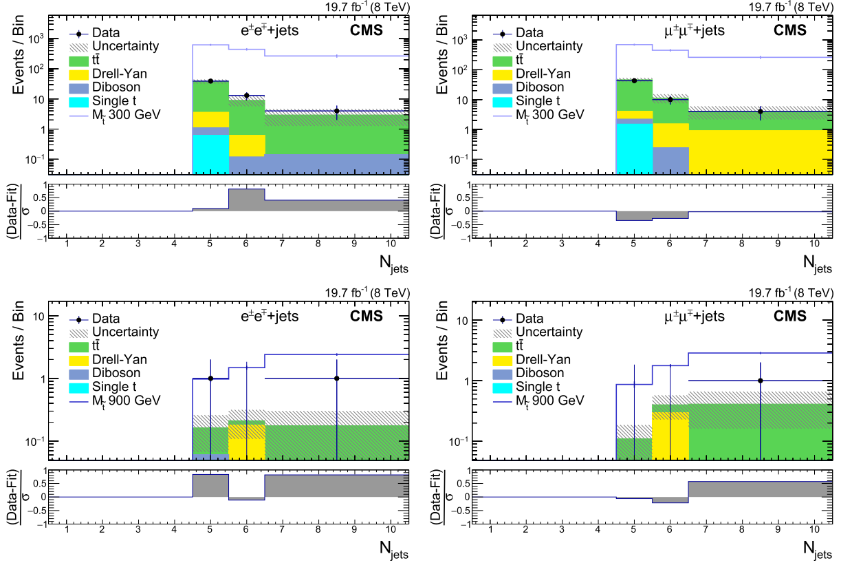
Fig. 2. Jet multiplicity distributions for e^+e^- (left) and \mu^+\mu^- (right) for selections optimized for M_{\tilde{t}} hypotheses of 300 GeV (top) and 900 GeV (bottom). The expected signal is shown by an open histogram superimposed on the expected SM background. The asymmetric error bars indicate the central confidence intervals for Poisson-distributed data. The systematic uncertainties for the SM contributions are indicated by hatched bands. Under each histogram is shown a plot in gray as the ratio of difference of data from background expectation to the sum of their uncertainties, including the systematic uncertainties in background expectation.
