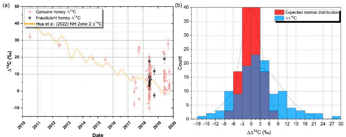
Fig. 3. Raw radiocarbon AMS results of honey samples from the USA (A) and the distribution of radiocarbon offset compared to the expected reference value from Hua et al. (2022) (b). The last available global background ^{14}\text{C}/^{12}\text{C} data is from early 2019, 0.01 \pm 0.83 ‰ ( \Delta^{14}\text{C} ). The reference value in Hua et al. (2022) is continuously decreasing due to the ocean-atmosphere and biosphere-atmosphere \text{CO}_2 exchange and fossil \text{CO}_2 emission. The red bars show the expected normal distribution, and the blue bars show the distribution of \Delta^{14}\text{C} offset compared to the expected reference value from Hua et al. (2022) (b).
