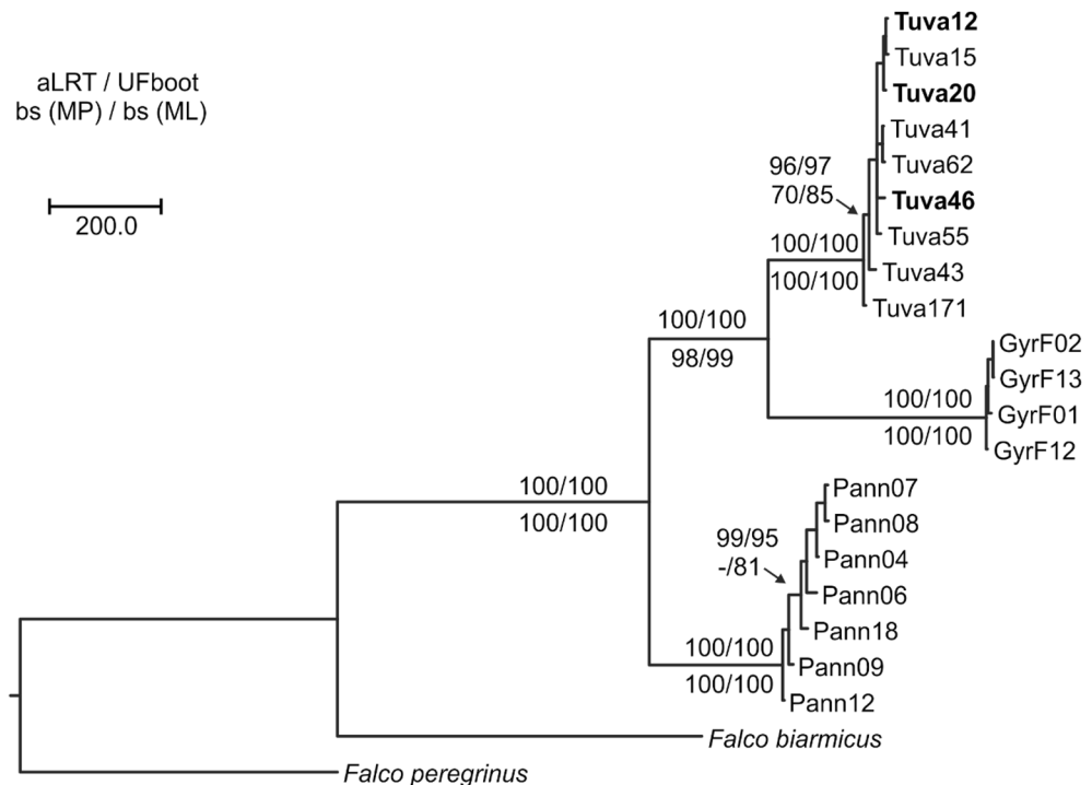
Figure 3. Phylogenetic tree based on phylogenetic analysis of concatenated data of 431 RAD loci with the inclusion of two outgroup samples, the lanner falcon ( Falco biarmicus ) as close, and the peregrine falcon ( F. peregrinus ) as distant outgroup species. The phylogenetic tree, displayed as a phylogram, is a representative one reconstructed by a maximum parsimony (MP) search that yielded 36 equally parsimonious trees. Topological robustness is indicated by displaying the branch support values coming from 1000 non-parametric bootstrap (bs) pseudo-replicates at the corresponding branches. The same data were used in a ML search that yielded a most likely phylogenetic tree with identical topology to the above shown one. Therefore, only support values resulting from SH-aLRT, UFboot and bs of the ML analysis are shown above at the corresponding branches. Branches that received support below 50 are not captioned. Sample names follow Table 1. Samples of the Altai falcon are indicated in boldface. The scale bar represents 200 mutation steps in the MP analysis.
