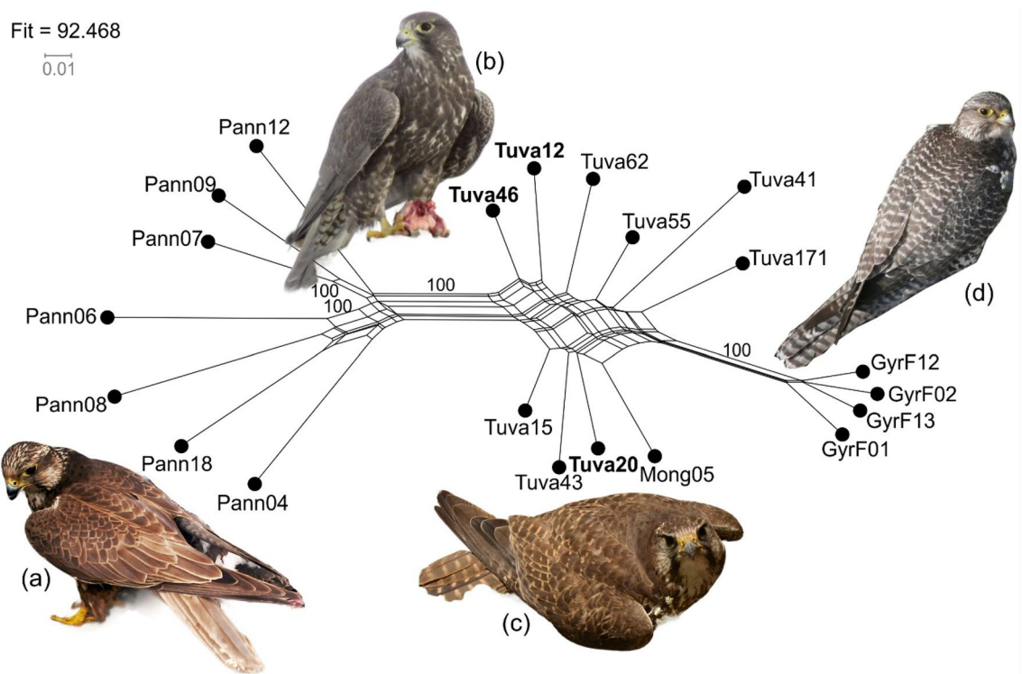
Figure 1. Genetic relationship between the studied saker falcon and gyrfalcon samples as depicted by a NeighbourNet network based on Kimura-2p genetic distance with non-parametric bootstrap (bs) support values built in SplitsTree. The numbers represent statistically significantly supported (bs > 75%) splits. Sample names follow Table 1. Samples of the ‘Altai falcon’ are indicated in boldface. Pictures of adult females of the studied taxa: (a) Falco cherrug cherrug (photo: János Bagyura), (b) Altai falcon (photo: Shane McPherson), (c) Falco cherrug milvipes (photo: Gábor Sramkó), (d) Falco rusticolus (photo: Alexander Sorokin).
