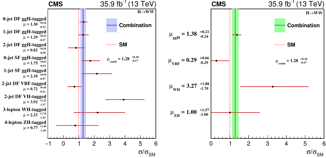
Fig. 9. (Left) Observed signal strength modifiers for the categories used in the combination. (Right) Observed signal strength modifiers corresponding to the main SM Higgs boson production mechanisms, for a Higgs boson with a mass of 125.09 GeV. The vertical continuous line represents the combined signal strength best fit value, while the horizontal bars and the filled area show the 68% confidence intervals. The vertical dashed line corresponds to the SM expectation.
