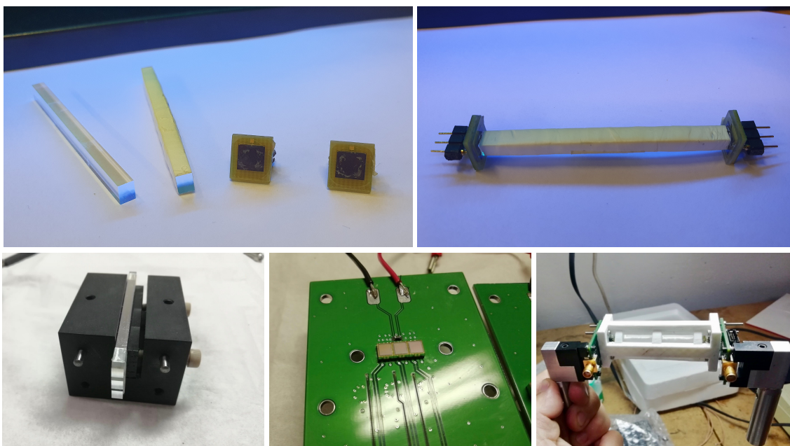
Figure 5. Top: naked and wrapped individual crystal bars with the two FBK SiPMs (left) and single wrapped bar glued to SiPMs (right). Bottom, from left to right: three-bar assembly in a crystal holder with the screws used to adjust the alignment of the crystals to the SiPMs on the readout board (left); HPK SiPMs soldered onto a readout board (middle); single bar assembly (right).
