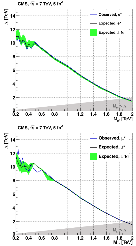
Fig. 5. Expected and observed 95% CL lower limits on the \Lambda scale for the different excited electron (top) and muon (bottom) mass points, using the \text{CL}_s method. The excluded region is below the curve. These limits are computed with the LO signal cross section obtained from PYTHIA 6.424. The one standard deviation uncertainty band is shown in green. The bands do not include the uncertainty on signal cross section. The grey area corresponds to the theoretically excluded region where M_{\ell^*} > \Lambda . (For interpretation of the references to color in this figure legend, the reader is referred to the web version of this Letter.)
