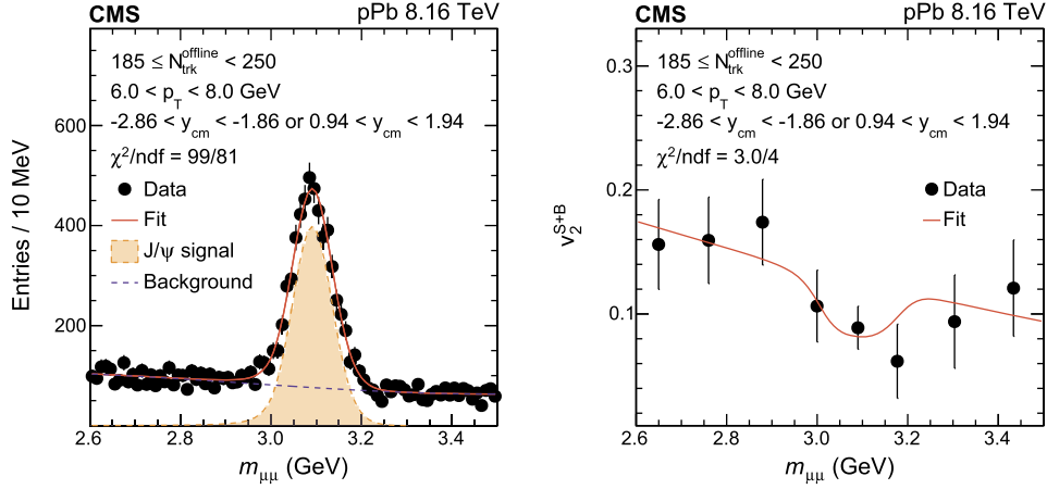
Fig. 1. Example of fits to the invariant mass spectrum (left) and the v_2^{S+B}(m_{\text{inv}}) distribution (right) in the p_T interval 6.0–8.0 GeV for pPb events with 185 \leq N_{\text{trk}}^{\text{offline}} < 250 .
