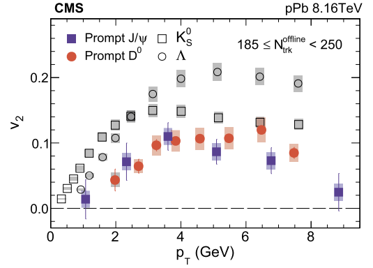
Fig. 2. The v_2 results of the prompt J/\psi mesons at forward rapidities ( -2.86 < y_{\text{cm}} < -1.86 or 0.94 < y_{\text{cm}} < 1.94 ), as a function of p_T in the multiplicity range 185 \leq N_{\text{trk}}^{\text{offline}} < 250 for pPb collisions at \sqrt{s_{\text{NN}}} = 8.16 TeV. Data for K_S^0 and \Lambda hadrons, and prompt D^0 mesons at midrapidity ( -1.46 < y_{\text{cm}} < 0.54 ) from previous CMS measurements [43] are also shown for comparison. The error bars correspond to statistical uncertainties, while the shaded areas denote the systematic uncertainties.
