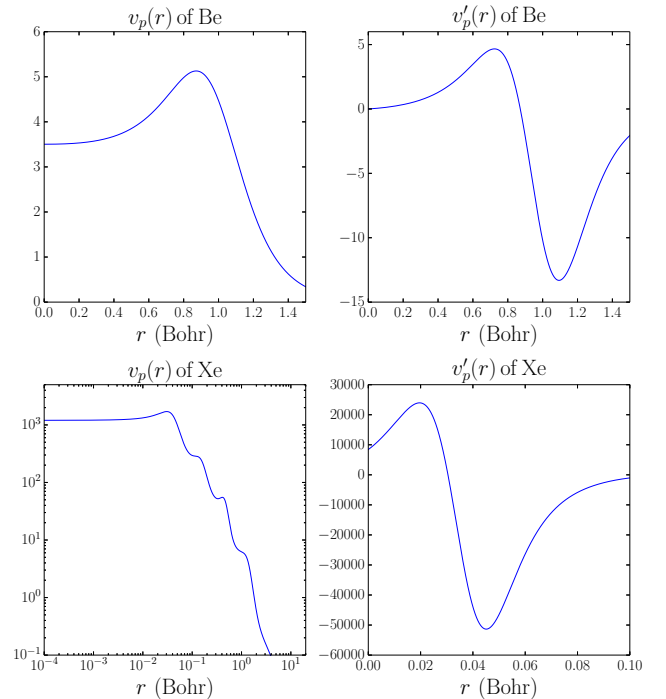
FIG. 1. Pauli potentials v_p(r) and their radial derivatives v'_p(r) (in atomic units) for Be and Xe atoms near the nucleus. They have been obtained from converged densities and Kohn-Sham potentials by inverting the Euler equation (6) for v_p(r) , that is, using Eq. (19). Values near the nucleus are seen to agree with those (Eqs. (29)- (30)) given in Table I.
