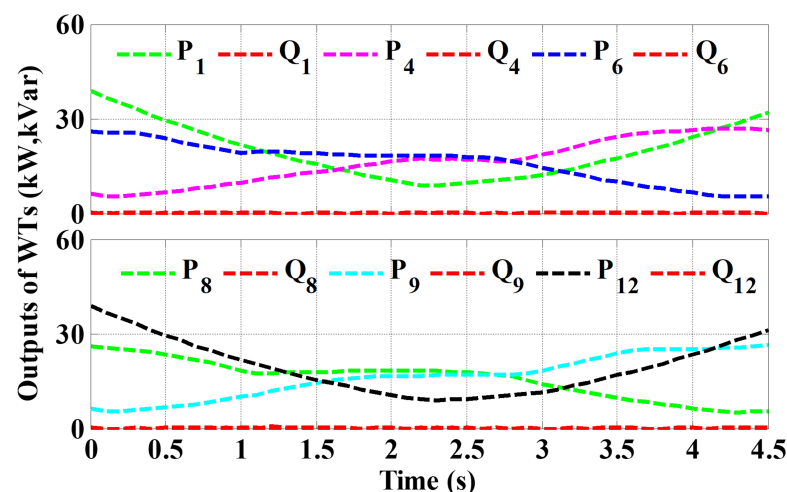
Figure 3. Power outputs of WTs.
