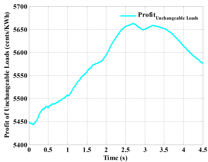
Figure 9. Profit of the unchangeable loads.
