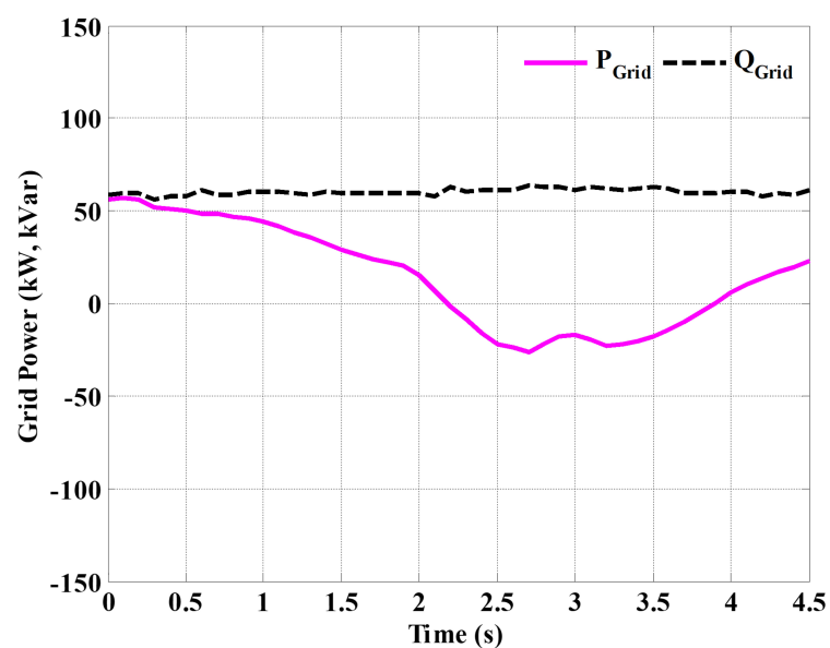
Figure 5. Power outputs of the main grid.
