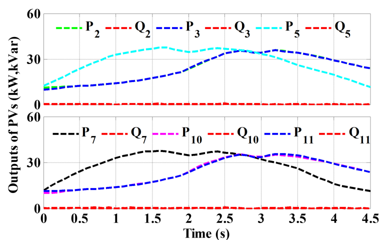
Figure 4. Power outputs of PVs.
