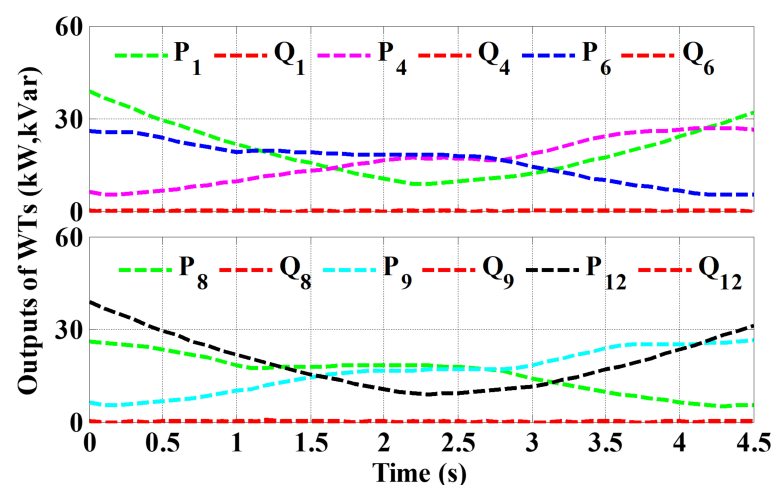
Figure 12. Power outputs of WTs.
