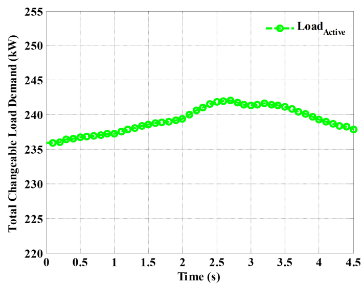
Figure 15. Total demand of changeable loads.
