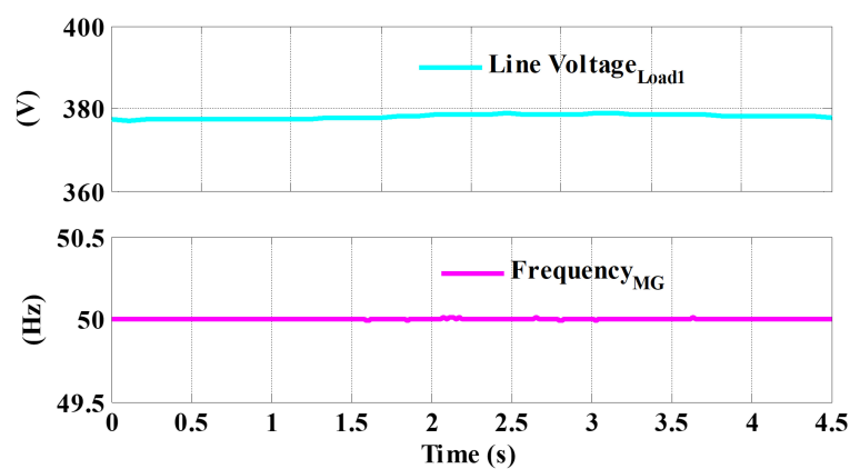
Figure 6. Line voltages and frequency in the MG.
