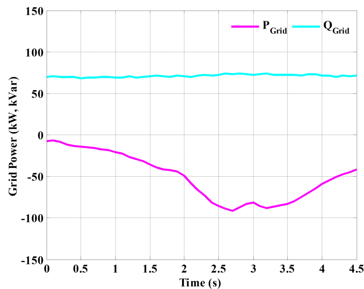
Figure 19. Power outputs of the main grid.
