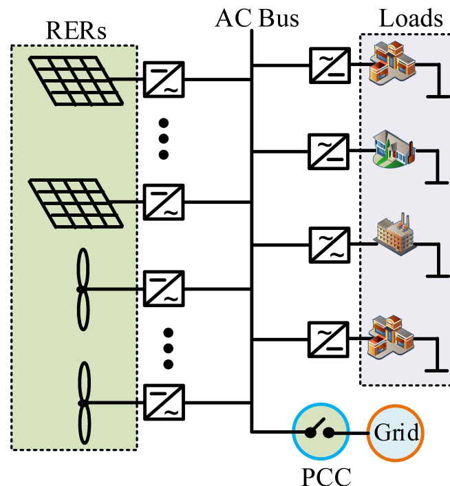
Figure 2. Grid-connected MG.
