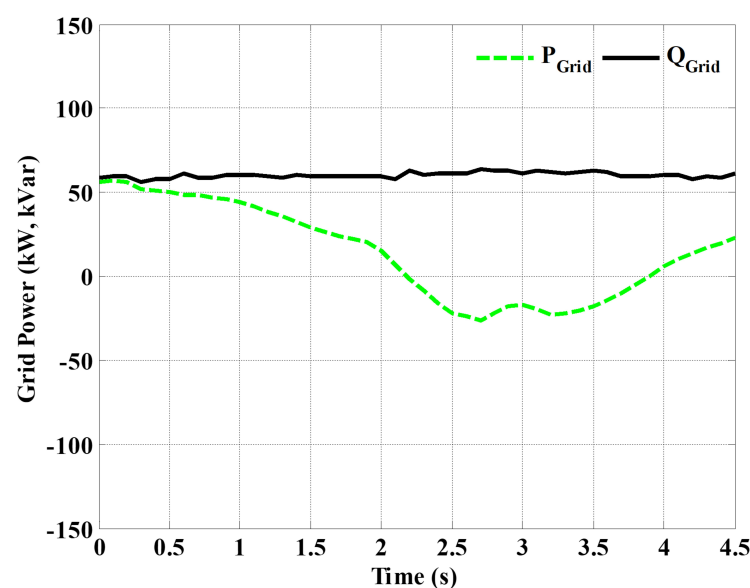
Figure 11. Power output of the main grid.
