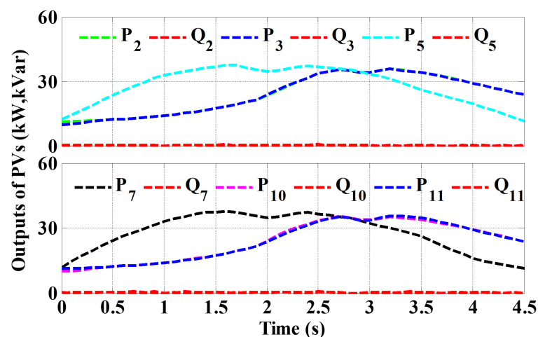
Figure 13. Power outputs of PVs.
