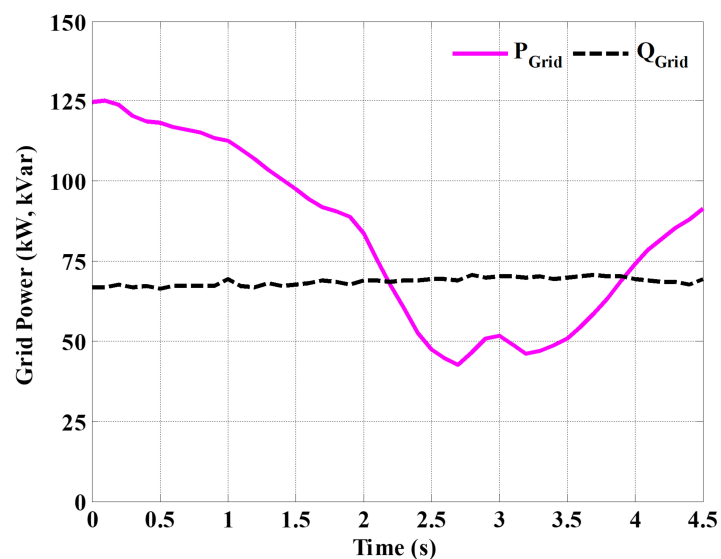
Figure 14. Power outputs of the main grid.
