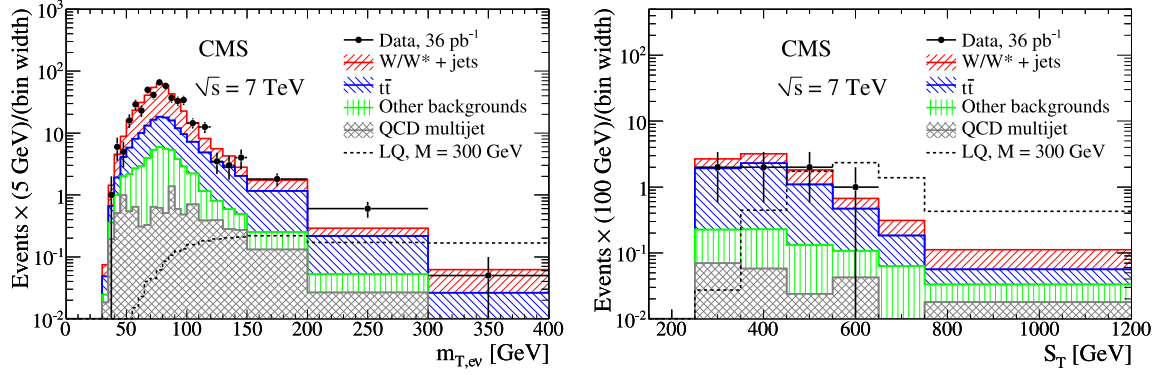
Fig. 1. (Left) The m_{T, ev} distribution for events passing the evjj preselection requirements. (Right) The S_T distribution for events passing the final evjj event selection except the optimized S_T cut itself ( S_T > 490 GeV for M_{LQ} = 300 GeV). The MC distributions for the signal ( M_{LQ} = 300 GeV, \beta = 0.5 ) and the contributing backgrounds listed in Section 4.1 are shown.
