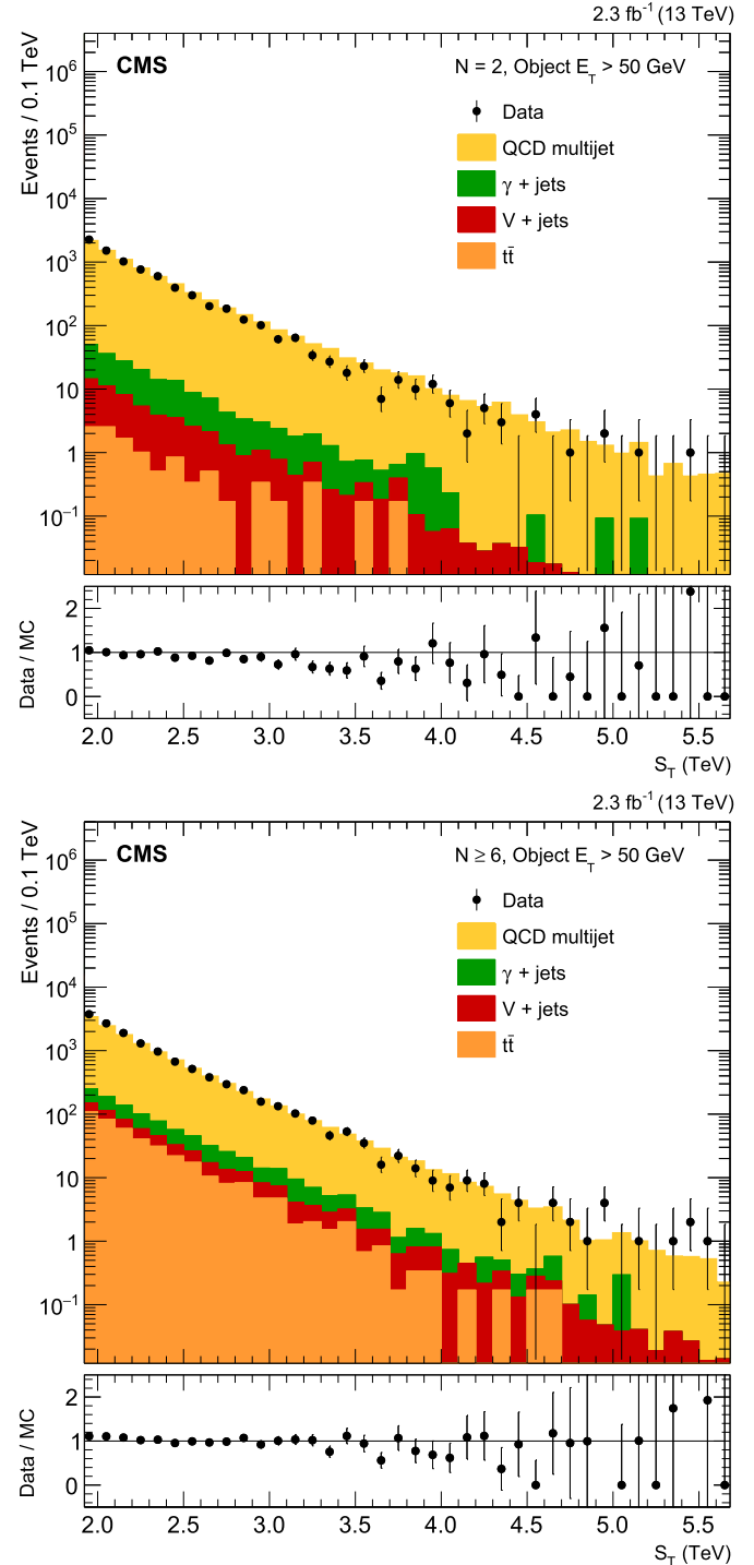
Fig. 1. Contributions of the main QCD multijet background, as well as \gamma + jets, V + jets ( V = W, Z ), and t\bar{t} backgrounds to the S_T distribution for (top) exclusive multiplicity N = 2 and (bottom) inclusive multiplicity N \geq 6 . All background predictions are based on simulated samples.
