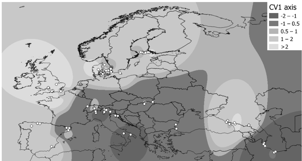
Figure 3. Inverse distance weighting (IDW) interpolation of the first CV axis. The CV1 axis can explain 40.91 % of the total variance between groups. Two main group are visible on the map: Northern group (brighter grey) and Southern group (darker grey). White dots indicate the collecting sites of the examined specimens. (Kiss et al. 2017a)
