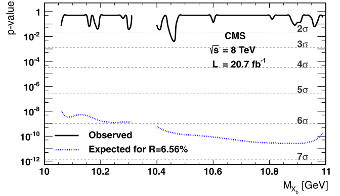
Fig. 3. Observed (solid curve) and expected for R = 6.56\% (dotted curve) local p-values, as a function of the assumed X_b mass.
