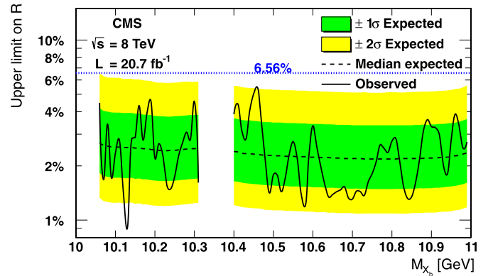
Fig. 4. Upper limits at the 95% confidence level on R , the production cross section for the X_b times its branching fraction to \Upsilon(1S)\pi^+\pi^- , relative to the \Upsilon(2S) , as a function of the X_b mass. The solid curve shows the observed limits, while the dashed curve represents the expected limits in the absence of a signal, with the two shaded regions giving the \pm 1 and \pm 2 standard deviation uncertainties on the expected limits. The measured value for the analogous X(3872) to \psi(2S) ratio of 6.56% is shown by the dotted line.
