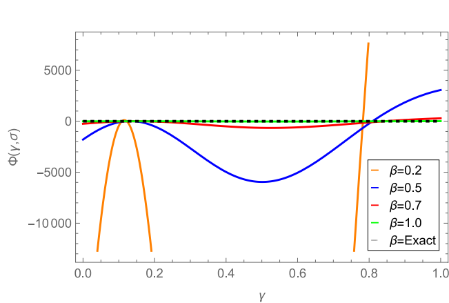
Fig. 7. Variations in \beta values and their impact on the fractional-order Sawada-Kotera equation with k = 1 and t = 0.1 set using NTIM.
