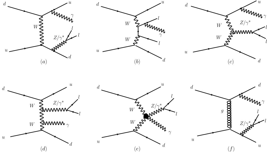
Fig. 1. Representative diagrams for EW Z\gamma\gamma production at the LHC: (a) bremsstrahlung, (b) multiperipheral, (c, d) VBF with TGC, (e) VBS including QGC, and (f) Example diagram for the QCD Z\gamma\gamma production.
