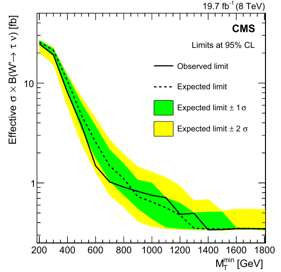
Fig. 5. Model independent limits, on the effective cross section for a W' -like signal above a threshold value M_T^{\min} , for different M_T^{\min} . The solid line shows the limit observed with 19.7 \text{ fb}^{-1} of data while the dashed line corresponds to the expected limit. The shaded bands indicate the 68% and 95% confidence intervals of the expected limit. The region above the curve is excluded.
