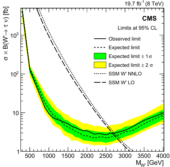
Fig. 3. Limits on the product of cross section and branching fraction into \tau \nu for a SSM W' boson. The solid line shows the limit observed with 19.7 \text{ fb}^{-1} of data while the dashed line corresponds to the expected limit. The shaded bands indicate the 68% and 95% confidence intervals of the expected limit. The dotted and the long-dashed lines show the cross section prediction in the SSM as a function of the W' boson mass, in NNLO and LO, respectively.
