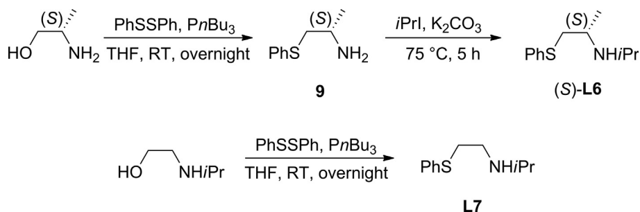
Scheme 7. Synthesis of ligands (S)-L6 and L7.
