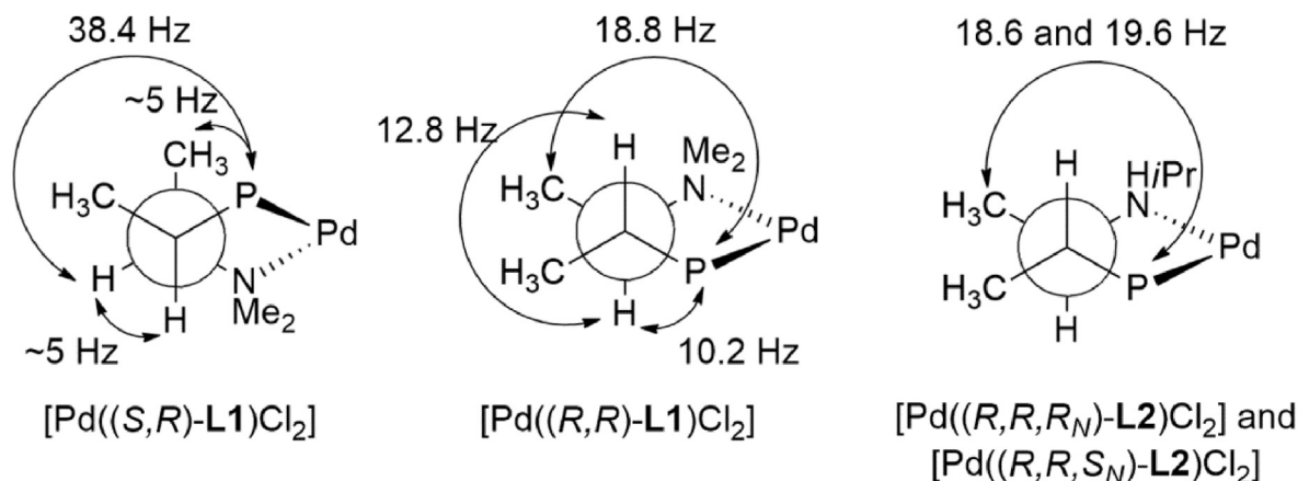
Fig. 3. Ring conformations of complexes [\text{Pd}((S,R)\text{-L1})\text{Cl}_2] , [\text{Pd}((R,R)\text{-L1})\text{Cl}_2] , [\text{Pd}((R,R,R_N)\text{-L2})\text{Cl}_2] and [\text{Pd}((R,R,S_N)\text{-L2})\text{Cl}_2] in solution. (The coupling constants were measured at room temperature using \text{CD}_2\text{Cl}_2 as solvent. The P-Ph substituents are omitted for clarity.)
