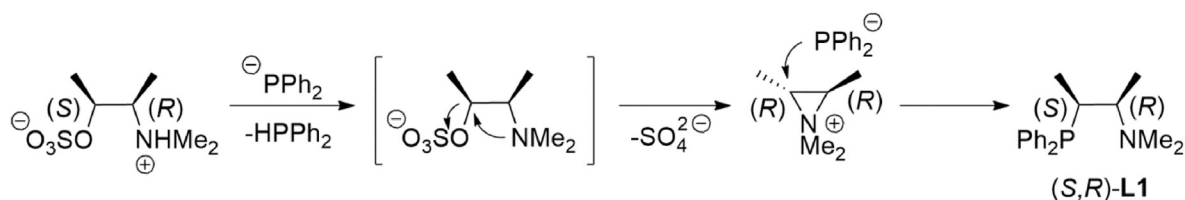
Scheme 2. Sequential double displacement leading to ligand ( S,R )- L1 .
