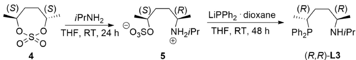
Scheme 3. Synthesis of ligand ( R,R )- L3 .
