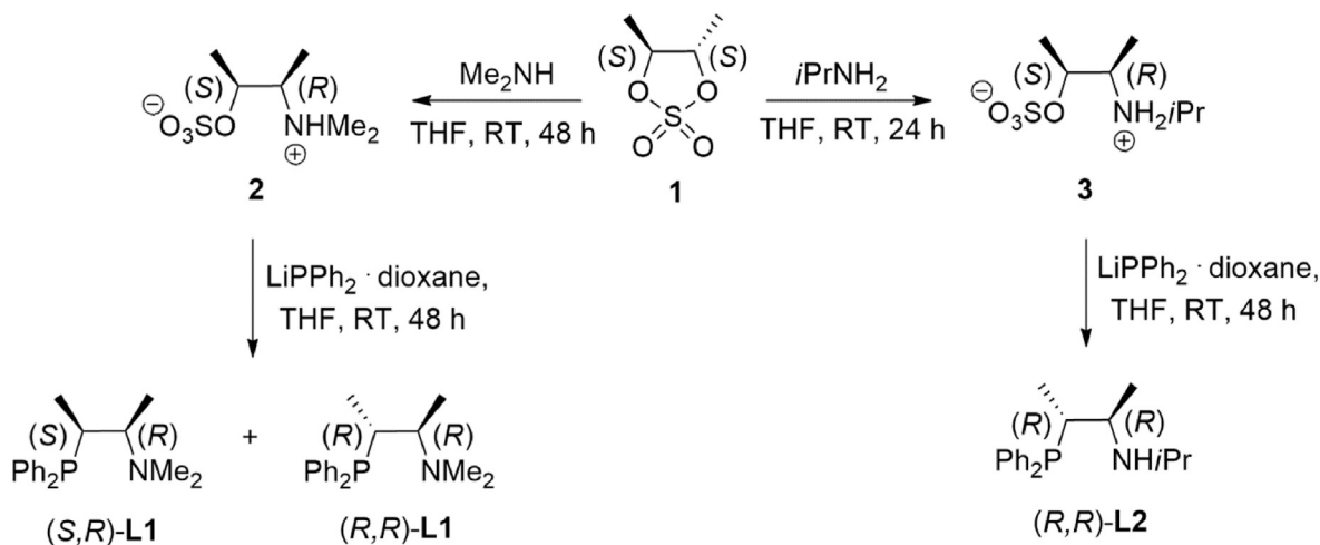
Scheme 1. Synthesis of chiral ligands ( S,R )- and ( R,R )- L1 and ( R,R )- L2 starting from cyclic sulfate 1 .
