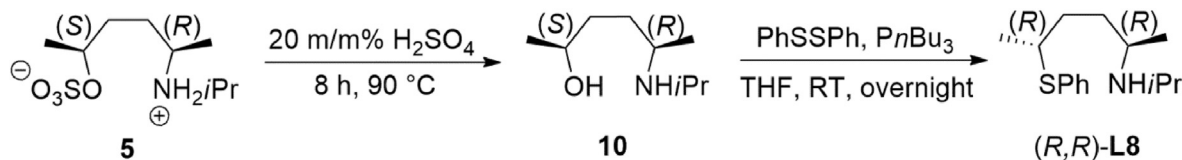
Scheme 8. Synthesis of ligand (R,R)-L8.
