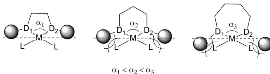
Fig. 4. Effect of bite angle on interligand interactions.
