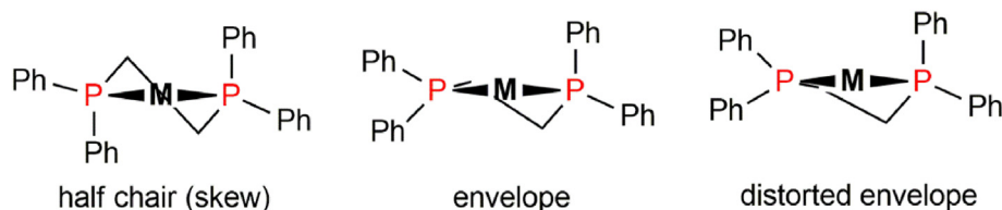
Fig. 1. Conformations of five-membered chelates. \lambda -skew (half chair), envelope and distorted envelope conformation of dppe metal-chelates.
