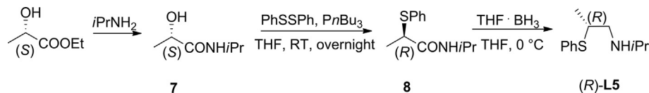
Scheme 6. Multistep synthesis of ( R )- L5 .
