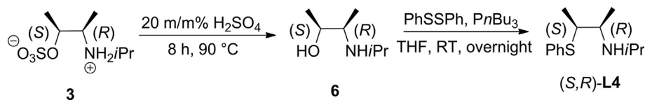
Scheme 4. Synthesis of ligand ( S,R )- L4 starting from the corresponding aminoalkyl sulfate 3 .
