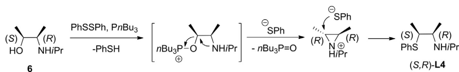
Scheme 5. Proposed mechanism for the stereoselective formation of ligand ( S,R )- L4 .
