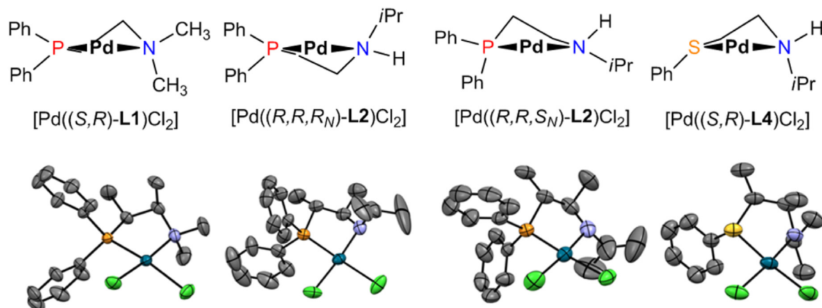
Fig. 2. Schematic and ORTEP views of five-membered chelates. (In schematic views the backbone methyl substituents and in the ORTEP views the hydrogens are omitted for clarity. The ORTEP views are depicted at 30% probability level.)
