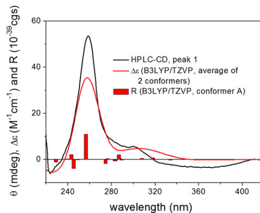
FIGURE 13 High-performance liquid chromatography-electronic circular dichroism (ECD) spectrum of the first-eluting enantiomer of 6 (black line) compared with the time-dependent density functional theory (DFT)-ECD spectrum of (3aR,4R) - 6 (red line: Boltzmann-weighted B3LYP/TZVP PCM/CHCl 3 ECD spectrum of the 2 low-energy solution conformers. Level of DFT optimization: B3LYP/TZVP PCM/CHCl 3 ). The bars represent rotational strength values for the lowest-energy solution conformer
