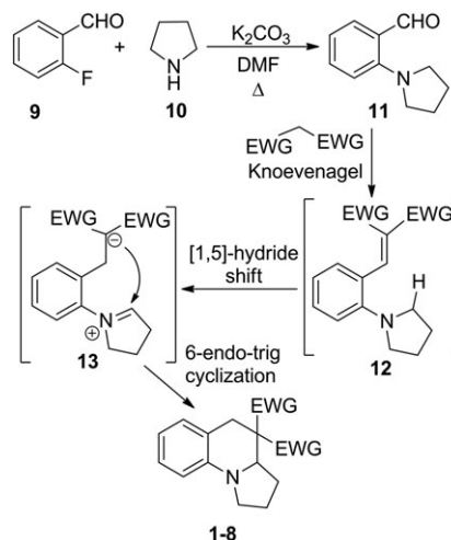
SCHEME 1 Preparation of the hexahydropyrrolo[1,2-a]quinoline derivatives 1 to 8 with the general mechanism of the domino reaction
