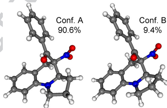
FIGURE 14 Low-energy conformers ( \geq 1\% ) of (3aR,4S) - 6 obtained at the B3LYP/TZVP PCM/CHCl 3 level of theory
