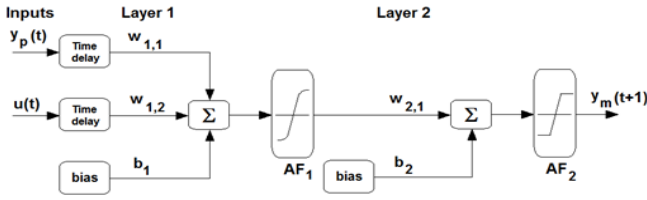
Fig.2. Neural model of the process.
