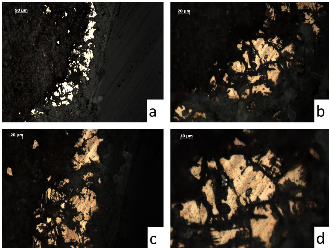
Fig. 14 Bright field optical micrographs of the sample of the dagger. Just a few metallic particles can be seen in the sample. Copper-sulphide inclusions can be observed between the metallic particles. Small lead inclusions are attached to the sulphide inclusions
