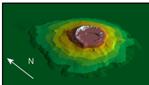
Figure 4. 3D DEM of the Haláp prepared on the basis of the 1:10000 topographic maps (1962-68) (Drawing: Molnár, L. Sz.)
