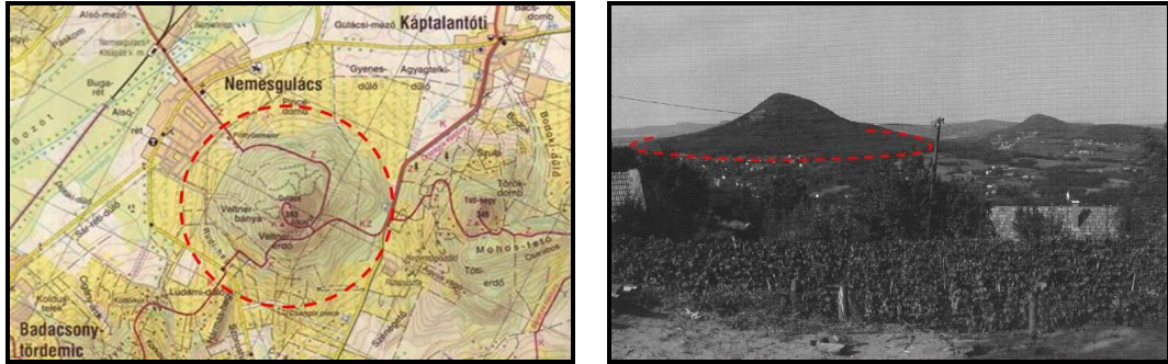
Figure 2. Same and still different: the Gulács on the tourist map with the scale of 1: 40 000 and in a traditional photo. Note: The dashed red line indicates the same area from different points of view. (Source: Cartographia Ltd. 2005; Molnár, L. 2007)
