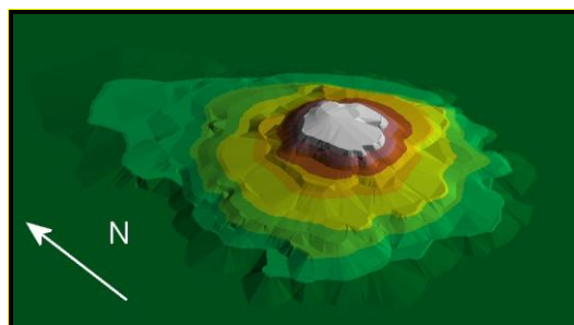
Figure 3. 3D DEM of the Haláp prepared on the basis of the Third Military Survey (1880-1881) (Drawing: Molnár, L. Sz.)
