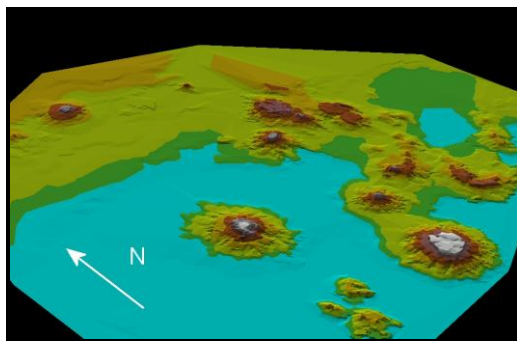
Figure 6. Reconstruction of the landscape prior to the water regulations based on the 130 m elevated shores (Drawing: Molnár, L. Sz.)
