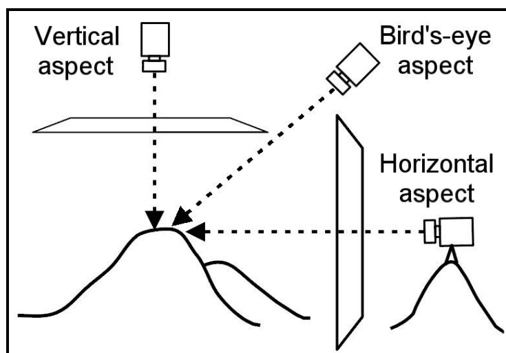
Figure 1. Problem of vertical and horizontal aspects in landscape research (Drawing: Molnár, L. Sz.)
