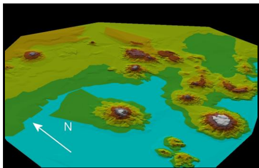
Figure 5. Reconstruction of the landscape prior to the water regulations based on the 120 m elevated shores (Drawing: Molnár, L. Sz.)
