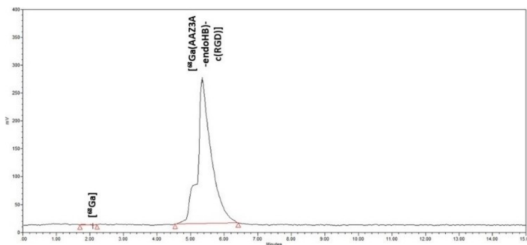
Figure 4. Radio-HPLC chromatogram of the purified [^{68}\text{Ga}(\text{AAZ3A-endoHB})\text{-c(RGD)}] probe. At 2.1 min there is a minimal fraction of free ^{68}\text{Ga} .
