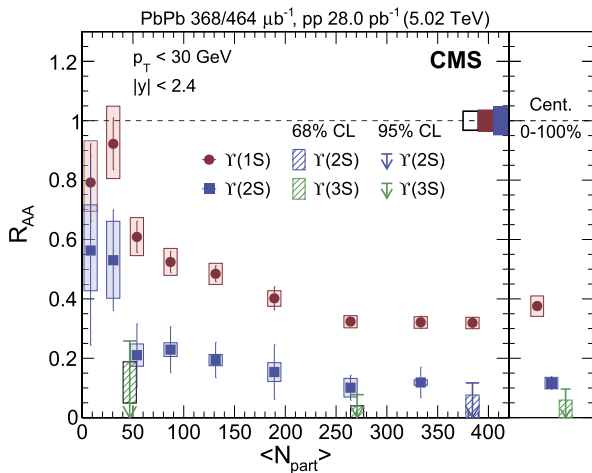
Fig. 5. Nuclear modification factors for the \Upsilon(1S) , \Upsilon(2S) and \Upsilon(3S) mesons as a function of \langle N_{part} \rangle . The boxes at the dashed line at unity represent global uncertainties: the open box for the integrated luminosity in pp collisions and N_{MB} in PbPb collisions, while the full boxes show the uncertainties of pp yields for \Upsilon(1S) and \Upsilon(2S) states (with the larger box corresponding to the excited state). For the \Upsilon(3S) meson, the upper limits at 68% (green box) and 95% (green arrow) CL are shown.
