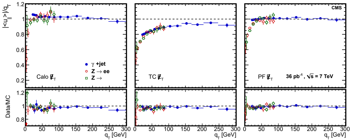
Figure 10. Response curves for events with one primary vertex, for (left) Calo \cancel{E}_T , (middle) TC \cancel{E}_T , and (right) PF \cancel{E}_T . Results are shown for photon events (full blue circles), Z \rightarrow e^+e^- events (open red circles) and Z \rightarrow \mu^+\mu^- events (open green squares). The upper frame of each figure shows the response in data; the lower frame shows the ratio of data to simulation. The vertical axis labels at the far left apply to all three subfigures.
