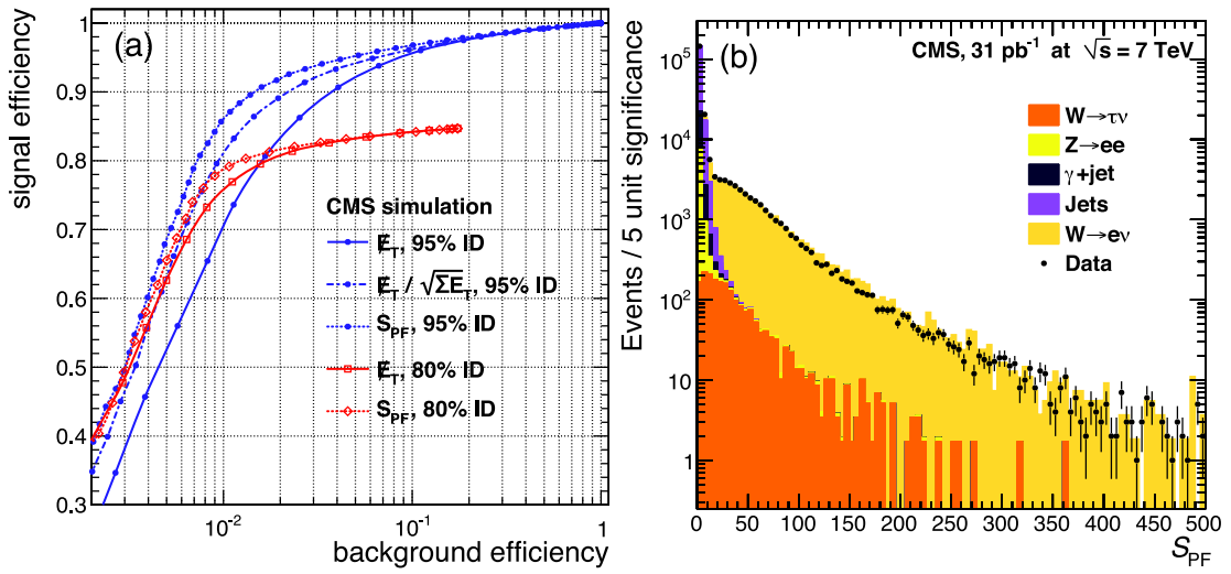
Figure 23. (left) Efficiency curves for W \rightarrow e\nu signal versus backgrounds varying the minimum value of \cancel{E}_T (solid lines), of S_{PF} (dotted lines), and of \cancel{E}_T/\sqrt{\sum E_{T_i}} (dot-dash line), with the 95% efficient (blue) or 80% efficient (red) electron isolation criterion applied. (right) Distributions of S_{PF} in candidate W \rightarrow e\nu events from data (points) and simulation (stacked histograms). The simulation components, from top to bottom, are signal (mustard) and backgrounds from jets (purple), \gamma +jets (black), Z \rightarrow e^+e^- (yellow), and W^\pm \rightarrow \tau^\pm\nu_\tau (orange). The simulation is scaled by a fit to the data with floating normalizations for the signal and the total background.
