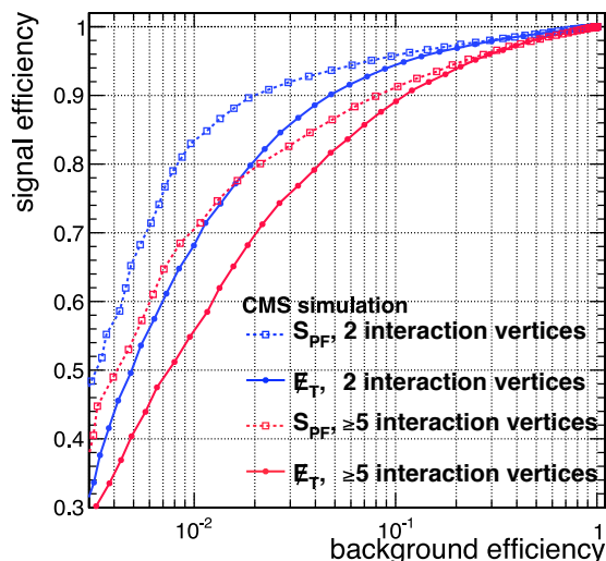
Figure 25. Efficiency curves for W \rightarrow e\nu signal versus backgrounds, varying the minimum value of \cancel{E}_T (solid lines) and of S_{PF} (dotted lines) for events with two interaction vertices (blue) or at least five interaction vertices (red).
