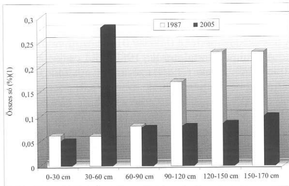
Figure 8: Saline content change in type meadow soil Total saline(‰)
