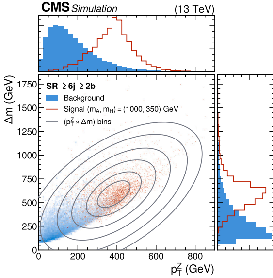
Fig. 2. Expected (\Delta m, p_T^Z) distribution for signal events with m_A = 1000 GeV and m_H = 350 GeV (red) and sum of backgrounds (blue) in the \text{SR } \geq 6j \geq 2b category, and boundaries of the elliptical bins (solid lines) used to construct the final observable.
