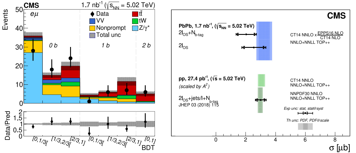
Fig. 66. Left: Observed and postfit predicted BDT discriminator distributions in the e^+\mu^\mp final state separately in the 0b-, 1b-, and 2b-tagged jet multiplicity categories. The data are shown with markers, and the signal and background processes with filled histograms. The vertical bars on the markers represent the statistical uncertainties in data. The hatched regions show the uncertainties in the sum of t\bar{t} signal and backgrounds. The lower panel displays the ratio between the data and the predictions, including the t\bar{t} signal, with bands representing the uncertainties in the postfit predictions. Right: Inclusive t\bar{t} cross sections measured with two methods in the combined e^+\mu^\mp , \mu^+\mu^- , and e^+e^- final states in PbPb collisions at \sqrt{s_{NN}} = 5.02 TeV, and pp results at \sqrt{s} = 5.02 TeV (scaled by A^2 ). The measurements are compared with theoretical predictions at NNLO+NNLL accuracy in QCD. The inner (outer) experimental uncertainty bars include statistical (statistical and systematic, added in quadrature) uncertainties. The inner (outer) theoretical uncertainty bands correspond to nPDF or PDF (PDF and scale, added in quadrature) uncertainties.
