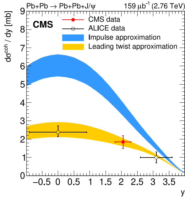
Fig. 28. Differential J/\psi meson photoproduction cross section as a function of rapidity in PbPb collisions at \sqrt{s_{NN}} = 2.76\text{ TeV} measured by ALICE [211,212] and CMS [213]. Data are compared with the leading twist [214] and the impulse approximation [214,215] predictions. The leading twist approximation is a perturbative QCD calculation that takes into account nuclear shadowing effects from multinucleon interference. Source: Figure adapted from Ref. [213].
