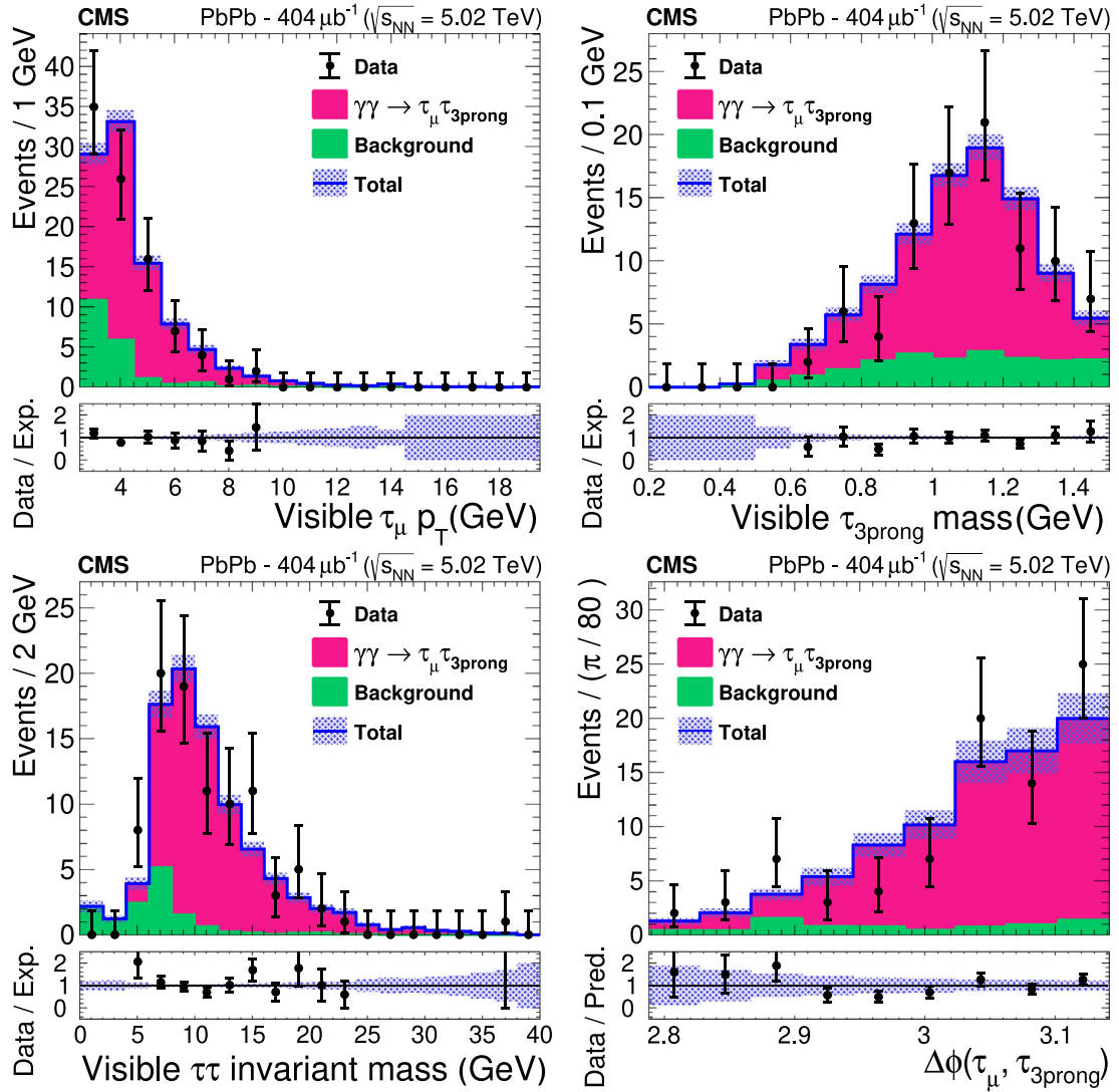
Fig. 108. Transverse momentum of the muon originating from the \tau_\mu candidate (upper left). Invariant mass of the three pions forming the \tau_{3\pi} candidate (upper right). Invariant mass of the \tau^+\tau^- system (lower left). The \Delta\phi(\tau_\mu, \tau_{3\pi}) azimuthal difference (lower right). In all plots, the signal component (magenta histogram) is stacked on top of the background component (green histogram). The sum of signal and background is displayed by a blue line and the shaded area shows the statistical uncertainty. The data are represented with black points and the uncertainty is statistical only. The lower panels show the ratios of data to the signal-plus-background prediction and the shaded bands represent the statistical uncertainty in the prefit expectation.
