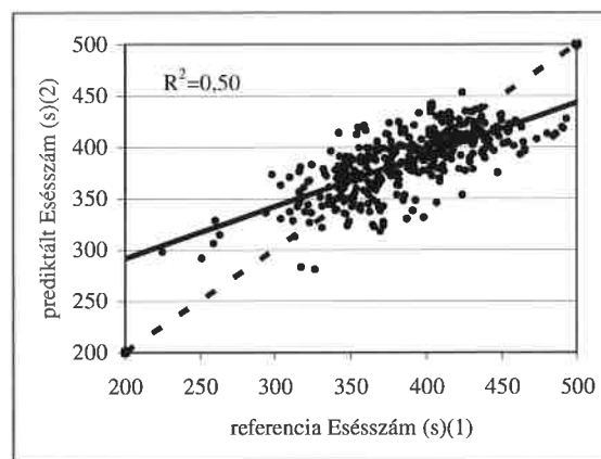
Figure 5: Comparison of falling number determined by prediction model and by reference method Falling number by reference method(1), Falling number predicted by the calibration modell(2)
