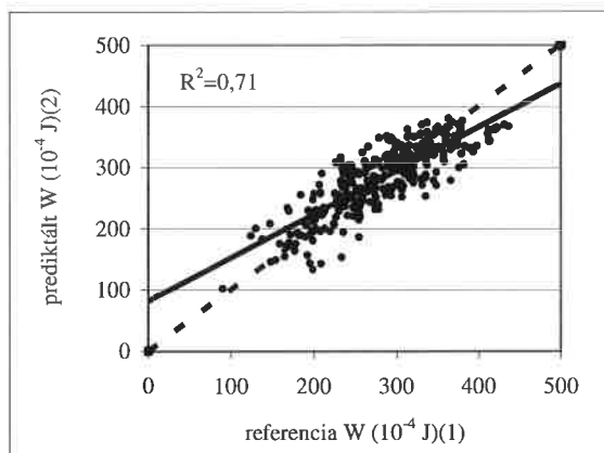
Figure 3: Comparison of W determined by prediction model and by reference method Alveographic W by reference method(1), Alveographic W predicted by the calibration modell(2)
