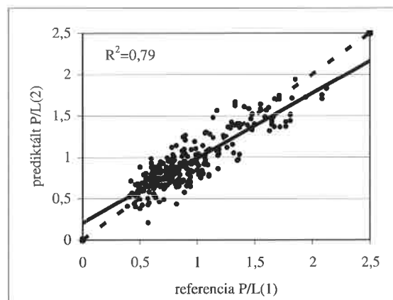
Figure 4: Comparison of P/L determined by prediction model and by reference method Alveographic P/L by reference method(1), Alveographic P/L predicted by the calibration modell(2)
