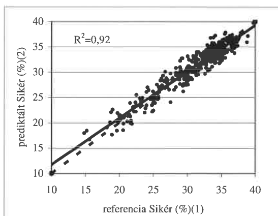
Figure 1: Comparison of gluten content determined by prediction model and by reference method Gluten content by reference method(1), Gluten content predicted by the calibration model(2)
