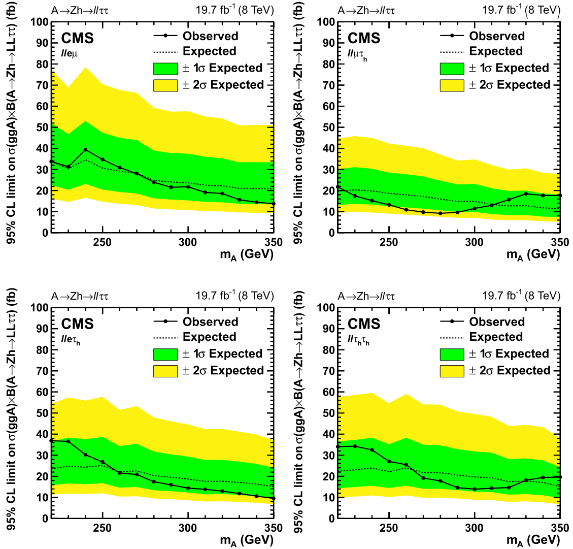
Fig. 9. Upper limits at 95% CL on cross section times branching fraction on A \rightarrow Zh \rightarrow LL\tau\tau for \ell\ell e\mu (top left), \ell\ell\mu\tau_h (top right), \ell\ell e\tau_h (bottom left), and \ell\ell\tau_h\tau_h (bottom right) final states.
