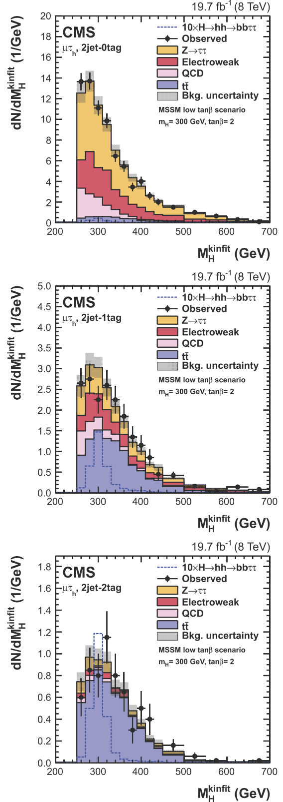
Fig. 3. Distributions of the reconstructed four-body mass with the kinematic fit after applying mass selections on m_{\tau\tau} and m_{b\bar{b}} in the \mu\tau_h channel. The plots are shown for events in the 2jet-0tag (top), 2jet-1tag (middle), and 2jet-2tag (bottom) categories. The expected signal scaled by a factor 10 is shown superimposed as an open dashed histogram for \tan\beta = 2 and m_H = 300 GeV in the low \tan\beta scenario of the MSSM. Expected background contributions are shown for the values of nuisance parameters (systematic uncertainties) obtained after fitting the signal plus background hypothesis to the data.
