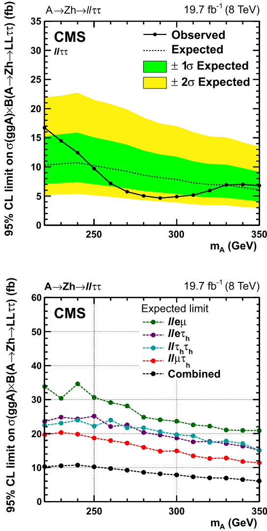
Fig. 10. Upper limits at 95% CL on cross section times branching fraction on A \rightarrow Zh \rightarrow \ell\ell\tau\tau for all \ell\ell\tau\tau final states combined (top) and comparison of the different final states (bottom).
