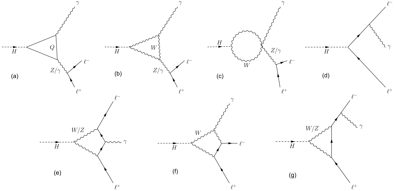
Fig. 1. Diagrams contributing to H \rightarrow \ell\ell\gamma . The contributions from diagrams (a), (b), and (c) dominate. The final-state radiation of H \rightarrow \mu\mu decay, shown in diagram (d), is important at high dilepton invariant mass. Higher order contributions from diagrams (e), (f) and (g) are negligible.
