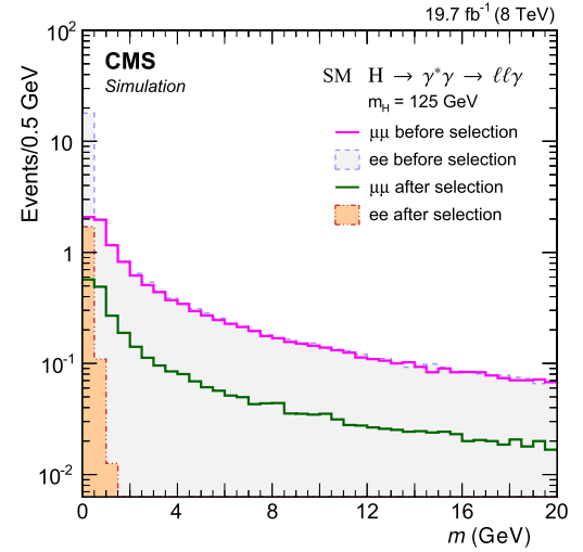
Fig. 3. The invariant mass of the dilepton system in signal simulation for m_H = 125 GeV. Distributions are shown for muon and electron channels, before and after selection. The invariant mass before selection is obtained from the leptons at the generator level, while after selection the reconstructed invariant mass is used.
