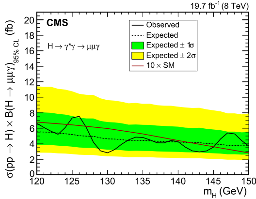
Fig. 7. The 95% CL exclusion limit on \sigma(\text{pp} \rightarrow \text{H})\mathcal{B}(\text{H} \rightarrow \mu\mu\gamma) , with m_{\mu\mu} < 20 GeV, for a Higgs-like particle, as a function of the mass hypothesis, m_{\text{H}} .
