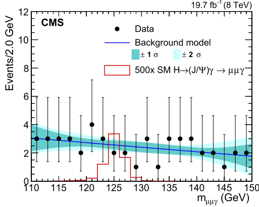
Fig. 5. The m_{\mu\mu\gamma} distribution for events with 2.9 < m_{\mu\mu} < 3.3 GeV for 8 TeV data (points with error bars), together with the result of a background-only fit to the data. The 1\sigma and 2\sigma uncertainty bands represent the uncertainty in the parameters of the fitted function. The expected contribution from the H \rightarrow (J/\psi)\gamma \rightarrow \mu\mu\gamma process of the SM H with m_H = 125 GeV, scaled up by a factor of 500, is shown as a histogram.
